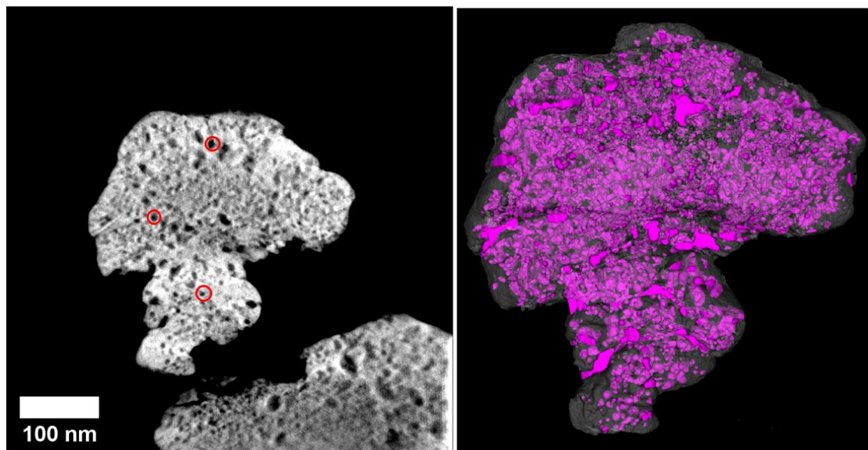
Figure 3 – Typical slice through the reconstruction (left) and the segmentation (right) of a palladium particle aged 6.5 years under tritium. For this tomography the tilting angles are between -78^\circ and +68^\circ . The size of the image is 667 \times 737 in pixel unit and the pixel size is 0.55 nm.
