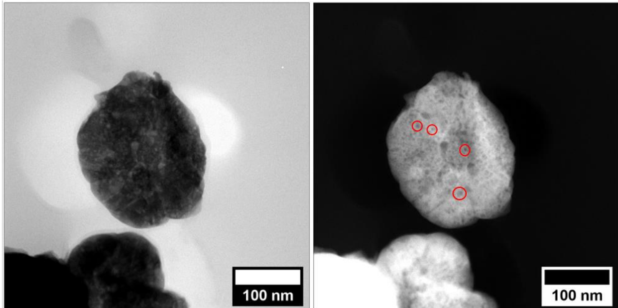
Figure 1 – Bright Field (left) and High Angle Annular Dark Field (right) images at 0^\circ tilt from the electron tomography series of palladium sample aged under tritium during five years. The pixel size is 0.45 nm. The image size is 1024x1024 in pixel unit.
