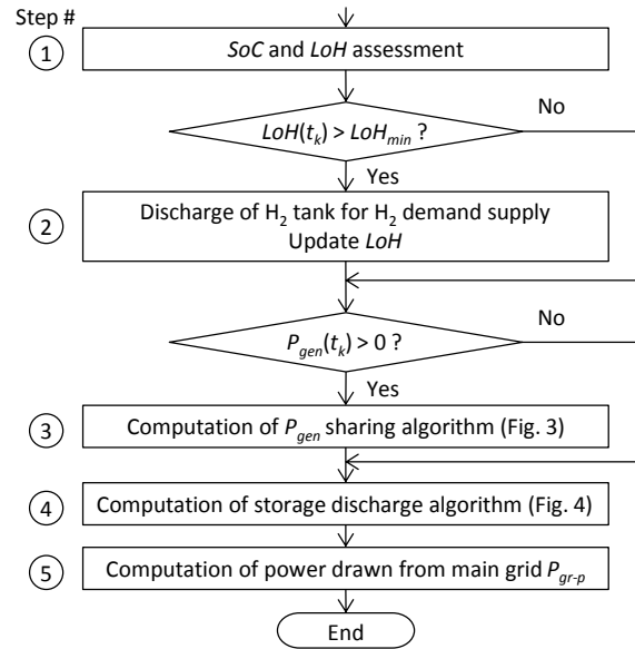
Fig. 2. Flowchart of the main algorithm applied at each time sample t_k
