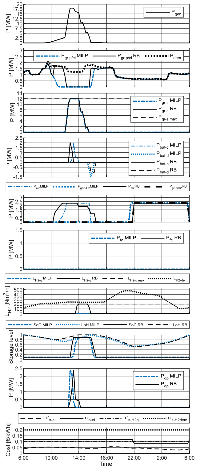
Fig. 5. Operating profiles for a one-day time window, obtained for MILP problem solving (blue curves) and rule-based algorithm (black curves)
