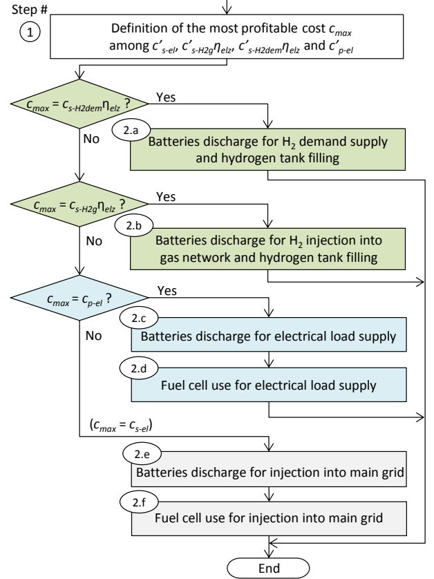
Fig. 4. Flowchart of the algorithm related to the discharge of the storage solutions
