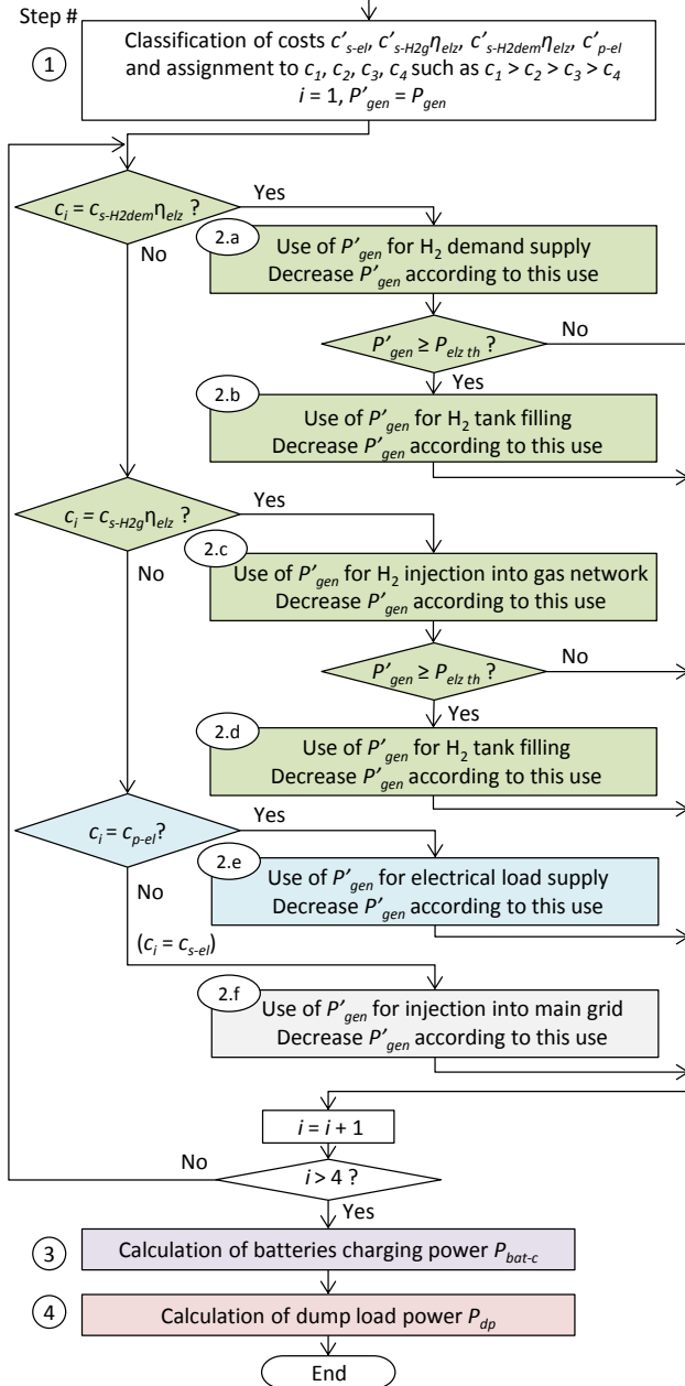
Fig. 3. Flowchart of the algorithm related to the power generated sharing
