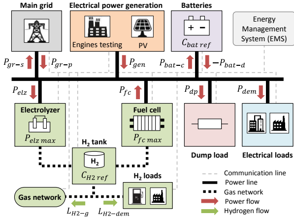
Fig. 1. Overview of the considered microgrid
