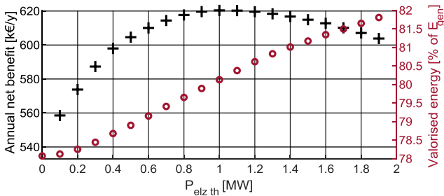
Fig. 6. Impact of electrolyzer power threshold P_{elz\ th} on the annual net profit (+ marker) and the valorised energy rate (o marker)
