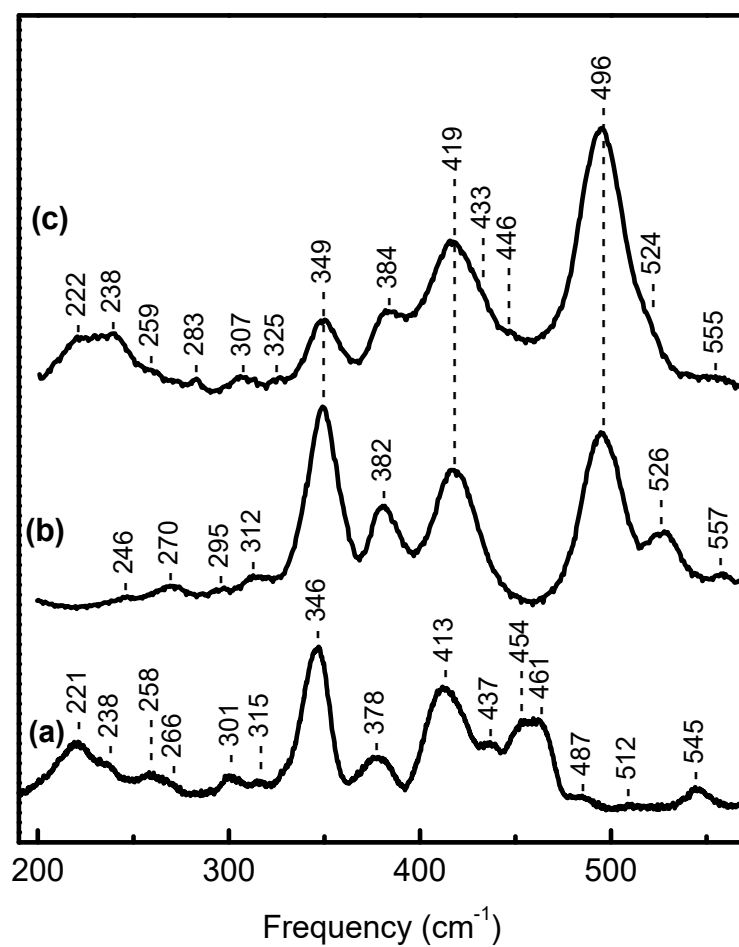
Figure 5. Low-frequency regions (190-570 \text{cm}^{-1} ) of RR spectra of ferroprothemo (Fe(II)PP) complexes of A \beta 40. (a) A \beta 40-Fe(II)PP complex excited at 441.6 nm; (b) A \beta 40-Fe(II)PPCO complex excited at 413.1 nm; (c) A \beta 40-Fe(II)PPCO complex excited at 441.6 nm.
