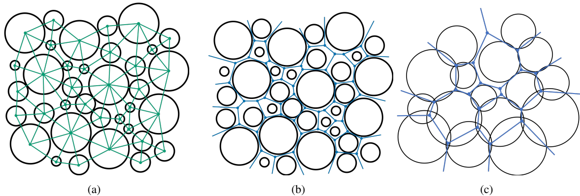
Figure 1: Tessellation of two-dimensional packings. (a) Regular Delaunay triangulation and its dual. (b) Radical Voronoi tessellation of a loose packing. (c) Radical Voronoi tessellation of a packing with overlaps. Figures adapted from [43, 44].
