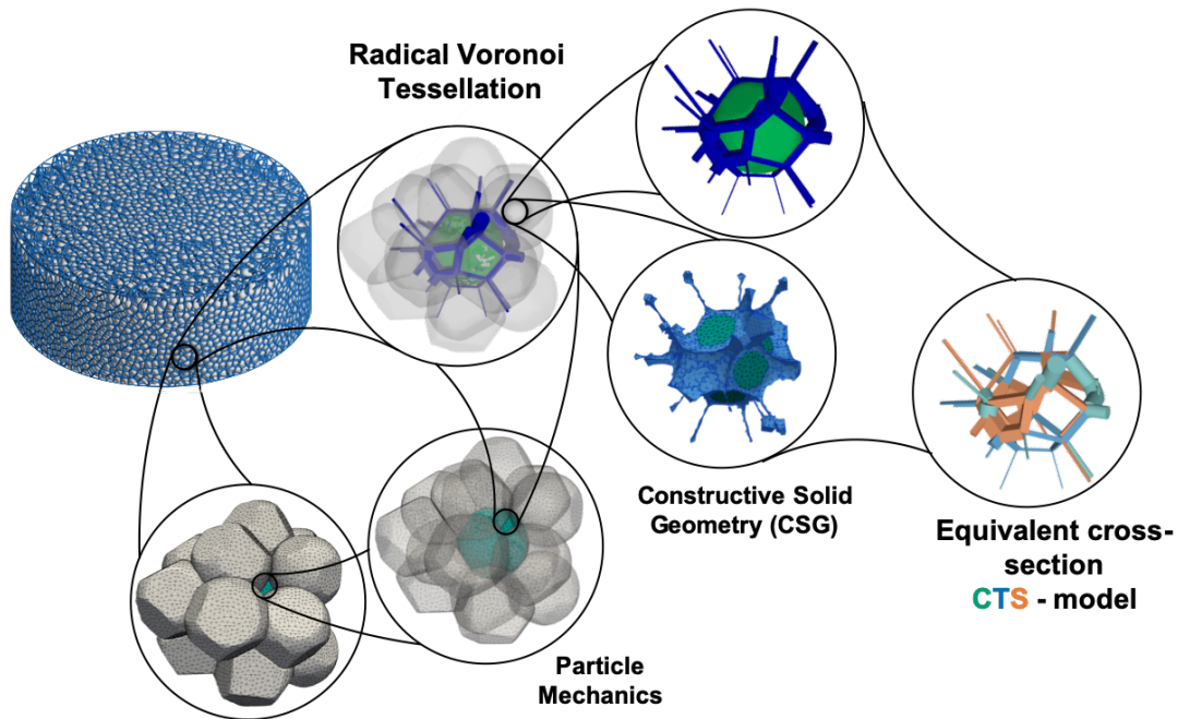
Figure 2: The process-based pore network model construction for granular packings under large plastic deformations is comprised of four key elements: (i) a particle mechanics approach to attain packings consolidated at large deformations, (ii) a tessellation algorithm to build the pore-network topology, (iii) CGS evaluations to generate pore geometry, and (iv) a CTS-model to assign transport properties to the pore network model.
