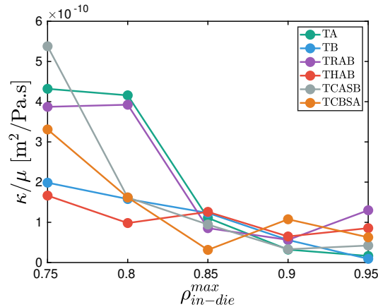
Figure 18: Effective permeability for all tablets listed in Table 4 under a pressure differential of \Delta P = 101,325 Pa between their top and bottom flat surfaces.
