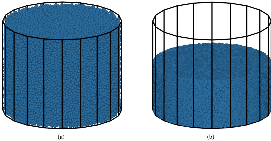
Figure 4: Compacted granular bed comprised of 39,914 weightless spherical particles, with Young’s modulus E = 5 GPa, Poisson’s ratio \nu = 0.25 , hardening stiffness \kappa = 150 MPa, hardening exponent m = 2 , and fracture toughness K_{Ic} = 1.26 MPa m 1/2 : (a) before compaction at a relative density, or solid fraction, of 0.5219, and (b) after compaction to a relative density of 0.9521.
