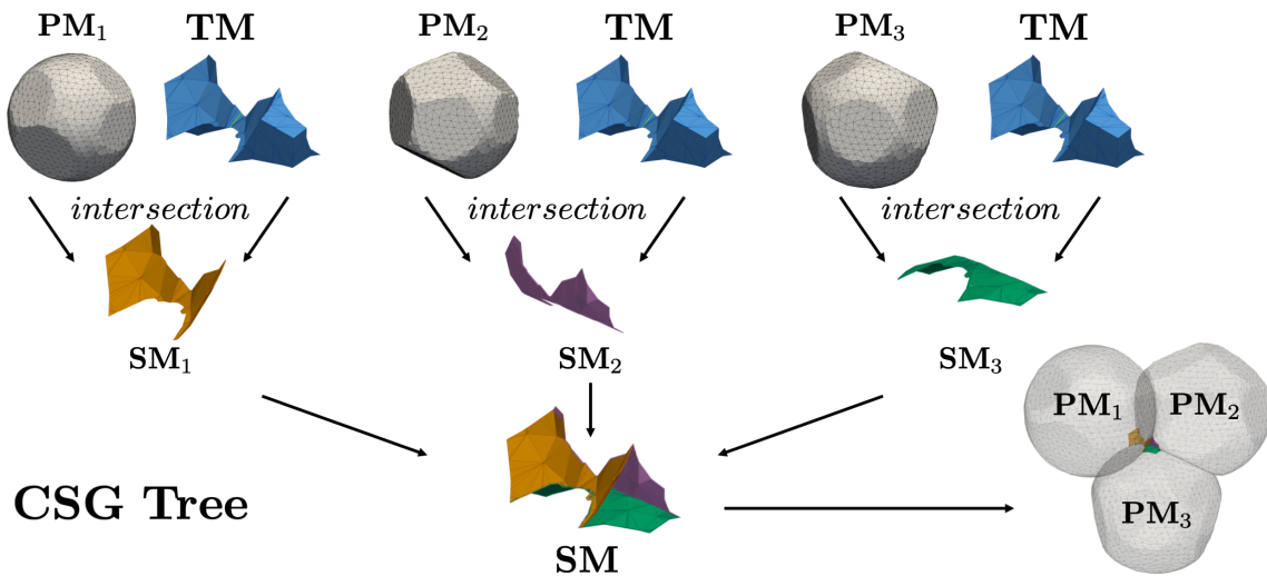
Figure 7: CSG tree for determining throat surface area S_t .
