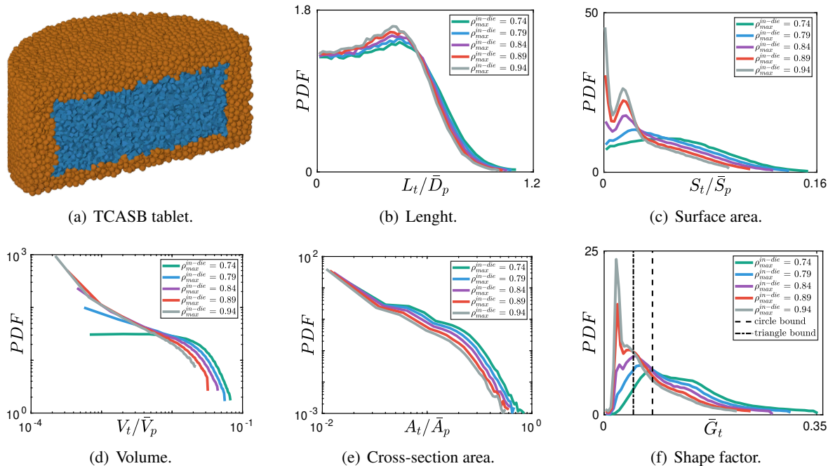
Figure 16: Pore-space statistical signature of the TCASB tablet.
