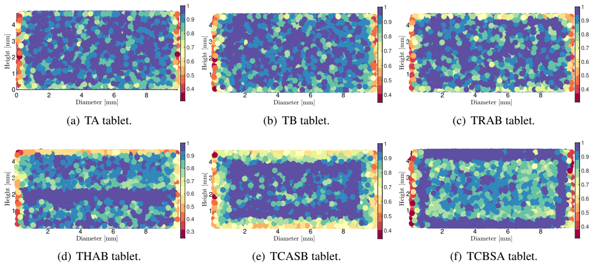
Figure 13: Internal distribution of relative density for tablets consolidated at a relative density of 0.904, unloaded and ejected from the die.
