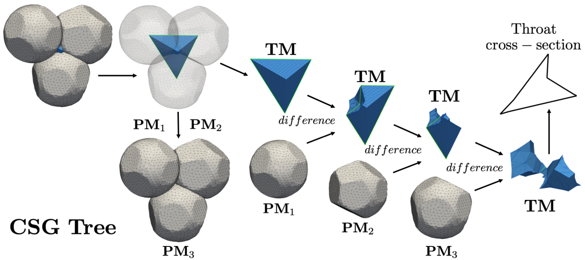
Figure 6: CSG tree for determining throat volume V_t and cross-section area A_t .
