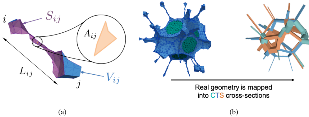
Figure 8: (a) Pore-space element geometric parameters, namely the throat cross-section area A_t , length L_t , surface area in contact with fluid S_t , and volume V_t . (b) Pore space (in blue) surrounding a particle (in green), and the equivalent CTS model.
