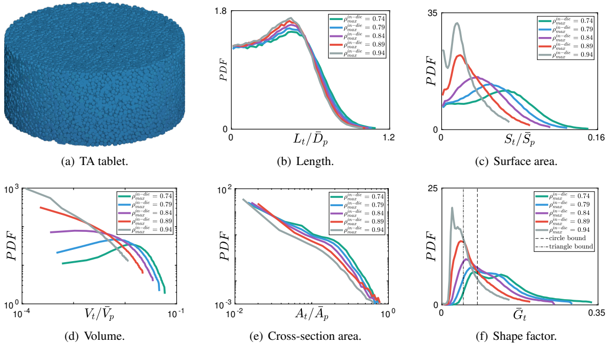
Figure 11: Pore-space statistical signature of the TA tablet.
