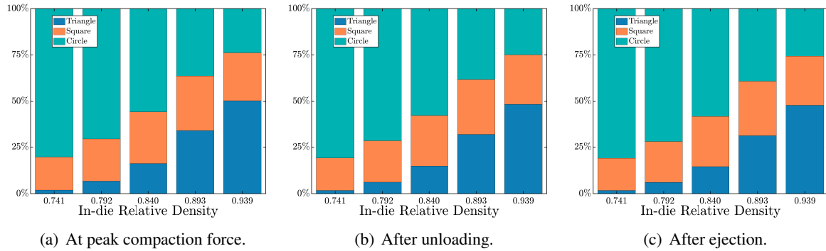
Figure 10: Evolution of pore-element equivalent shape during consolidation of granular packings under large deformations.
