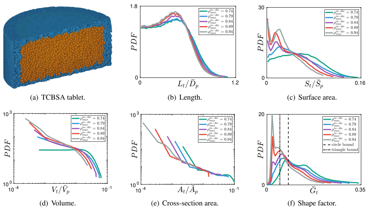
Figure 17: Pore-space statistical signature of the TCBSA tablet.
