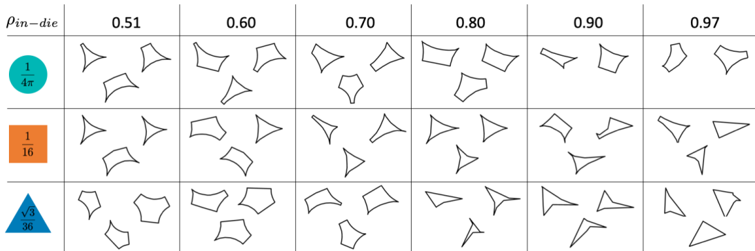
Figure 9: Examples of arbitrarily selected cross-sections that illustrate the CTS model mapping and the evolution of pore network properties during consolidation of granular packings under large deformations.
