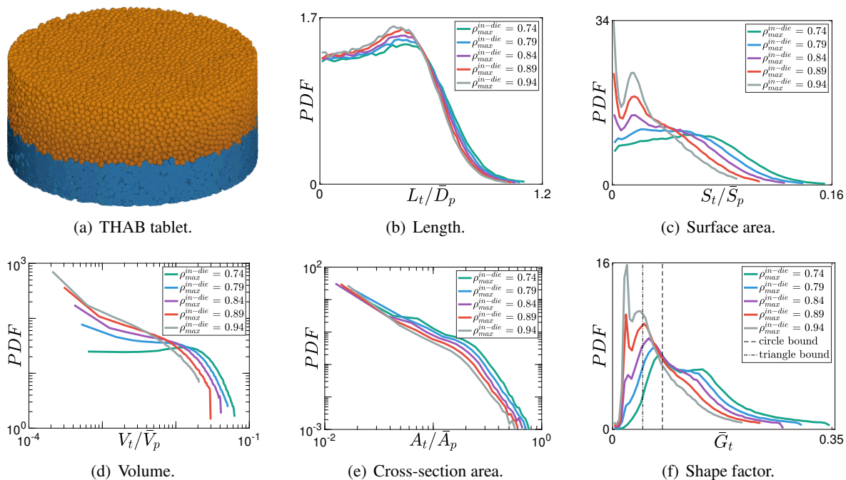
Figure 15: Pore-space statistical signature of the THAB tablet.
