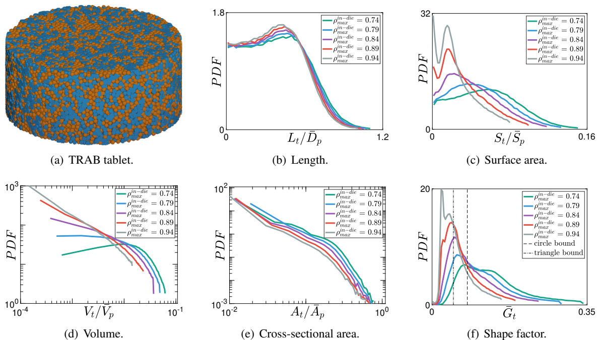
Figure 14: Pore-space statistical signature of the TRAB tablet.
