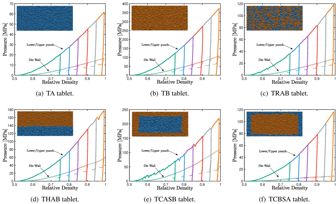
Figure 12: Punch and die-wall pressures as a function of relative density for tablets unloaded at six different levels of consolidation \rho_{\max}^{\text{in-die}} = [0.751, 0.805, 0.854, 0.904, 0.952, 0.998] .
