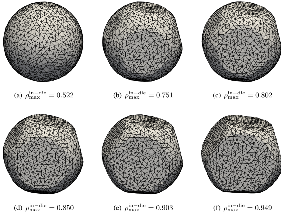
Figure 5: Deformed configuration of an arbitrarily selected particle, as the granular bed is deformed at different in-die relative densities, namely \rho_{\max}^{\text{in-die}} = [0.522, 0.751, 0.802, 0.850, 0.903, 0.949] . The granular bed and corresponded material properties are shown in Figure 4.
