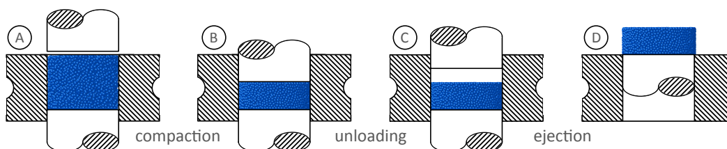
Figure 3: Consolidation of the granular packing during the stages of die compaction: (A) die filling, (B) compaction, (C) unloading, and (D) tablet ejection. Adapted from [50].
