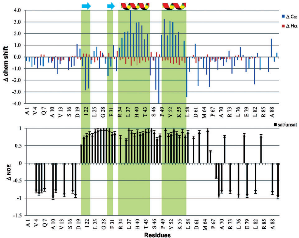
Fig. 6. (Top) Bar plot of C \alpha and H \alpha chemical-shift deviations from their random-coil values ( \delta observed – \delta random coil) as a function of residue number for Ros87_RGF protein. Secondary structure fragments are indicated. (Bottom) Bar plot of heteronuclear NOE values of Ros87_RGF protein. h-NOE values for some residues were not presented because of resonance overlap.
