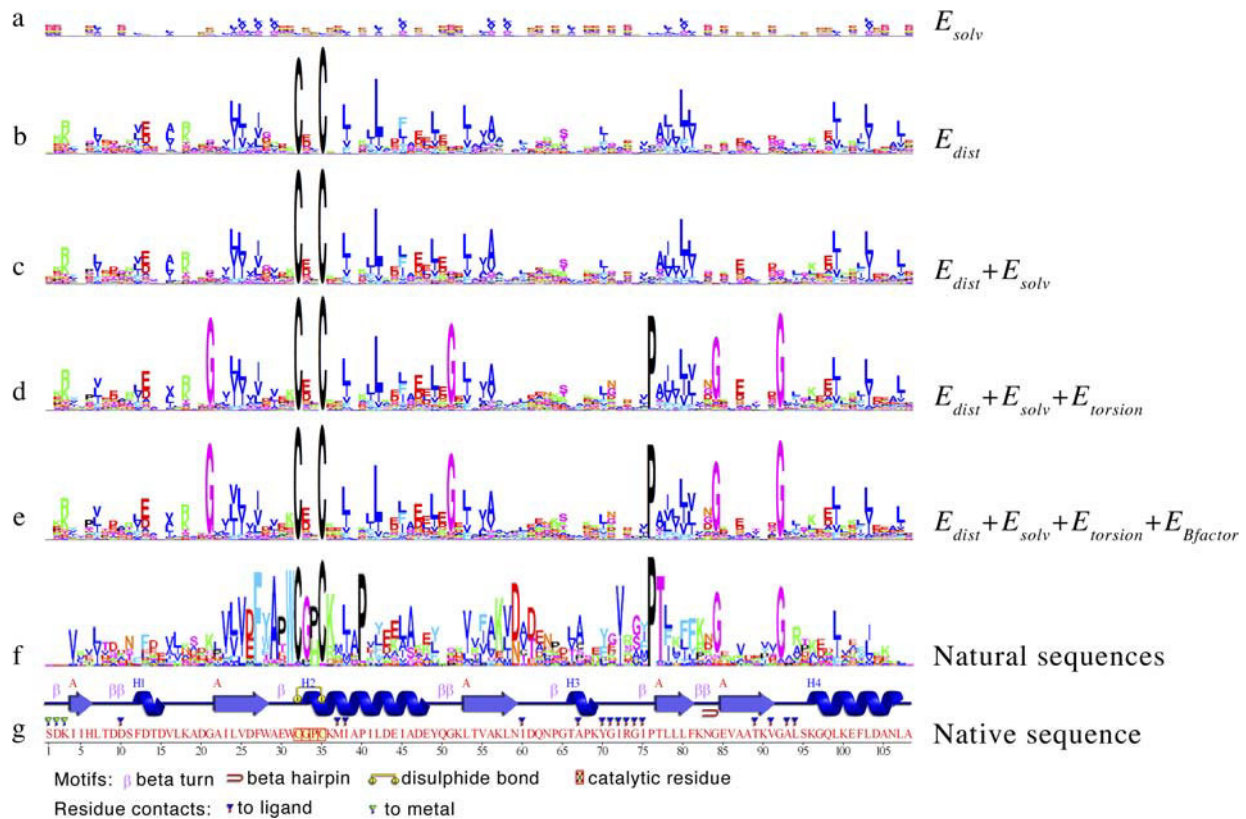
FIG. 4. Sequence logos of site-specific profiles induced on a thioredoxin (PDB: 2TRX, chain A), using the potentials (a) E_{solv} , (b) E_{dist} , (c) E_{dist,solv} , (d) E_{dist,solv,torsion} , and (e) E_{dist,solv,torsion,Bfactor} . (f) Profile obtained from a multiple sequence alignment of 162 eukaryotic sequences. (g) Native sequence of the reference protein. Secondary structure representation from PDBsum (Laskowski 2009). A color version of this figure is available as supplementary material, Supplementary Material online.
