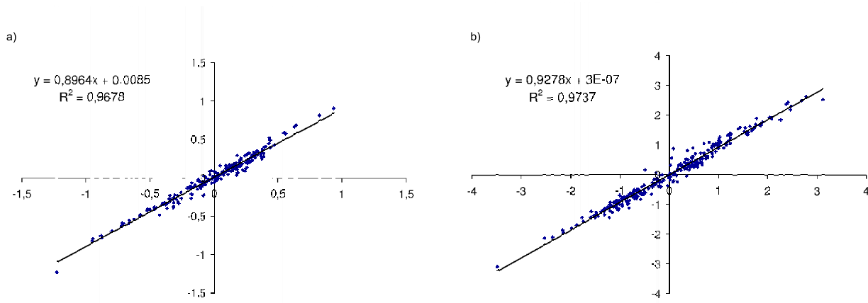
Figure 4 XY comparisons of the leave-one-out and joint potential parameters. XY comparisons between the two potentials (optimized on the same dataset DS_j ), with, in X-axis the leave-one-out potential, and in Y-axis the joint potential. (a) represents the correlation between the contact potential parameters, and (b) the correlation between the accessibility potential parameters.
