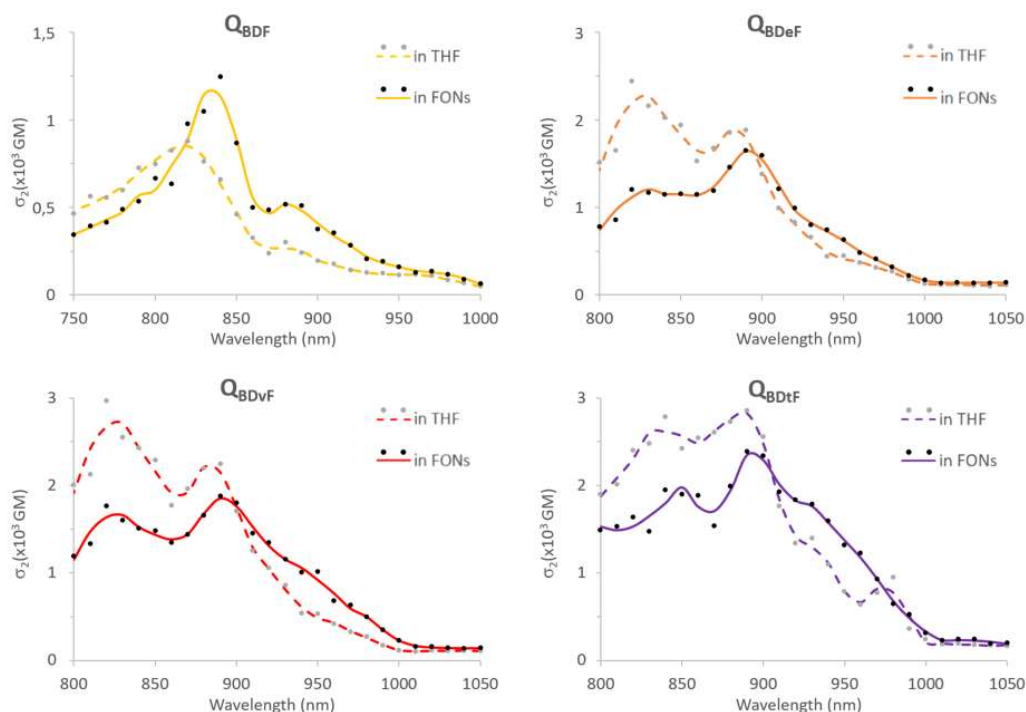
Figure 4. Non-linear properties of the dyes in THF (dashed lines) and in FONs (solid lines).
