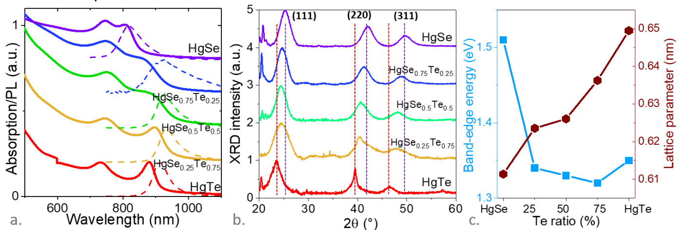
Figure 3: Spectroscopic and structural properties of alloyed \text{HgSe}_{1-x}\text{Te}_x NPLs. a. Absorption (solid lines) and PL (dashed lines) spectra of \text{HgSe}_{1-x}\text{Te}_x NPLs with various compositions. For the sake of clarity, the spectra of various compositions have been vertically shifted. b. X-ray diffraction pattern for a film made of \text{HgSe}_{1-x}\text{Te}_x NPLs with various compositions. For the sake of clarity, the diffractograms of various compositions have been vertically shifted. Vertical dashed lines are here as guide lines of the peak positions for zinc blende HgTe (red lines) and HgSe (blue lines) of lattice parameters a_{\text{HgTe}}=0.65 nm and a_{\text{HgSe}}=0.61 nm. c. Band-edge energy and lattice parameter of HgSeTe NPLs as a function of the Te content.
