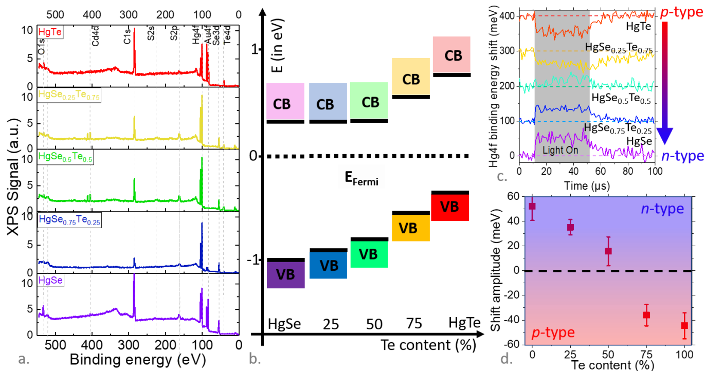
Figure 5: Electronic properties of \text{HgSe}_{1-x}\text{Te}_x NPLs with various compositions. a. X-ray photoemission overview spectra for \text{HgSe}_{1-x}\text{Te}_x NPLs with various compositions. Analysis of the core levels are given in Figure S8. b. Band alignment of the \text{HgSe}_{1-x}\text{Te}_x NPLs with various compositions. Analysis of the valence bands are given in Figure S12. c. Temporal shift of the binding energy of the Hg4f states from \text{HgSe}_{1-x}\text{Te}_x NPLs with various compositions, followed by XPS while sample is illuminated by a pulse of light at 405 nm. The dashed lines are base lines. d. Shift of the Hg 4f binding energy measured by TrXPS as a function of the Te content for \text{HgSe}_{1-x}\text{Te}_x NPLs.
