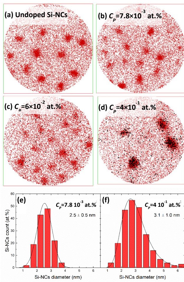
Fig. 2. 2D slice view ( 21 \times 21 \times 3 \text{ nm}^3 ) taken from the 3D reconstructed volume showing both Si (red points) and P (black points) atoms for (\text{SiO}/\text{SiO}_2):\text{P} multilayers annealed at 1100 \text{ }^\circ\text{C} with (a) C_p = 0 \text{ at.}\% , (b) C_p = 7.8 \times 10^{-3} \text{ at.}\% , (c) C_p = 6 \times 10^{-2} \text{ at.}\% and (d) C_p = 4 \times 10^{-1} \text{ at.}\% . Lower panel shows size dispersion of Si-NCs obtained from (\text{SiO}/\text{SiO}_2):\text{P} multilayer with (e) C_p = 7.8 \times 10^{-3} \text{ at.}\% , and (f) C_p = 4 \times 10^{-1} \text{ at.}\% , respectively.
