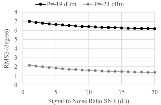
Fig. 5. AoA RMSE at the test frequency 61 GHz
