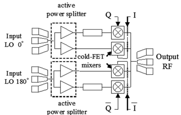
Fig. 1. Synoptic of the overall MMIC topology
