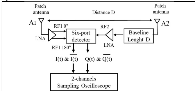
Fig. 4. MMIC-based receiver for AoA / TDoA configuration
