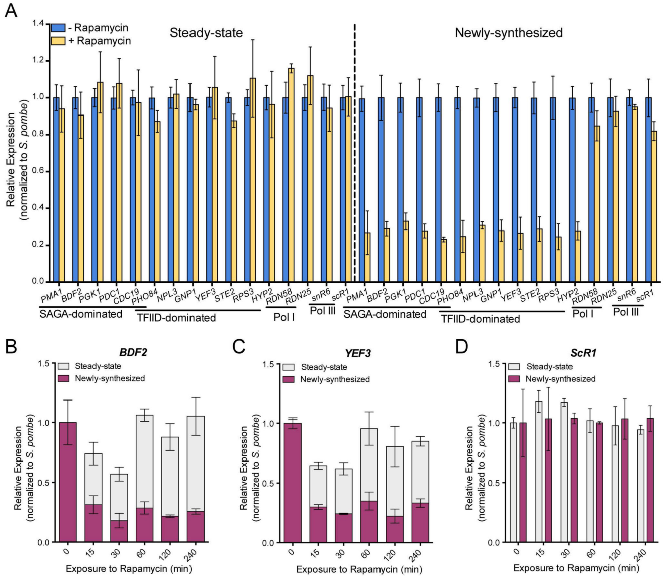
Figure 5. Conditional nuclear depletion of Spt7 decreased transcription of both SAGA- and TFIIID-dominated genes.
