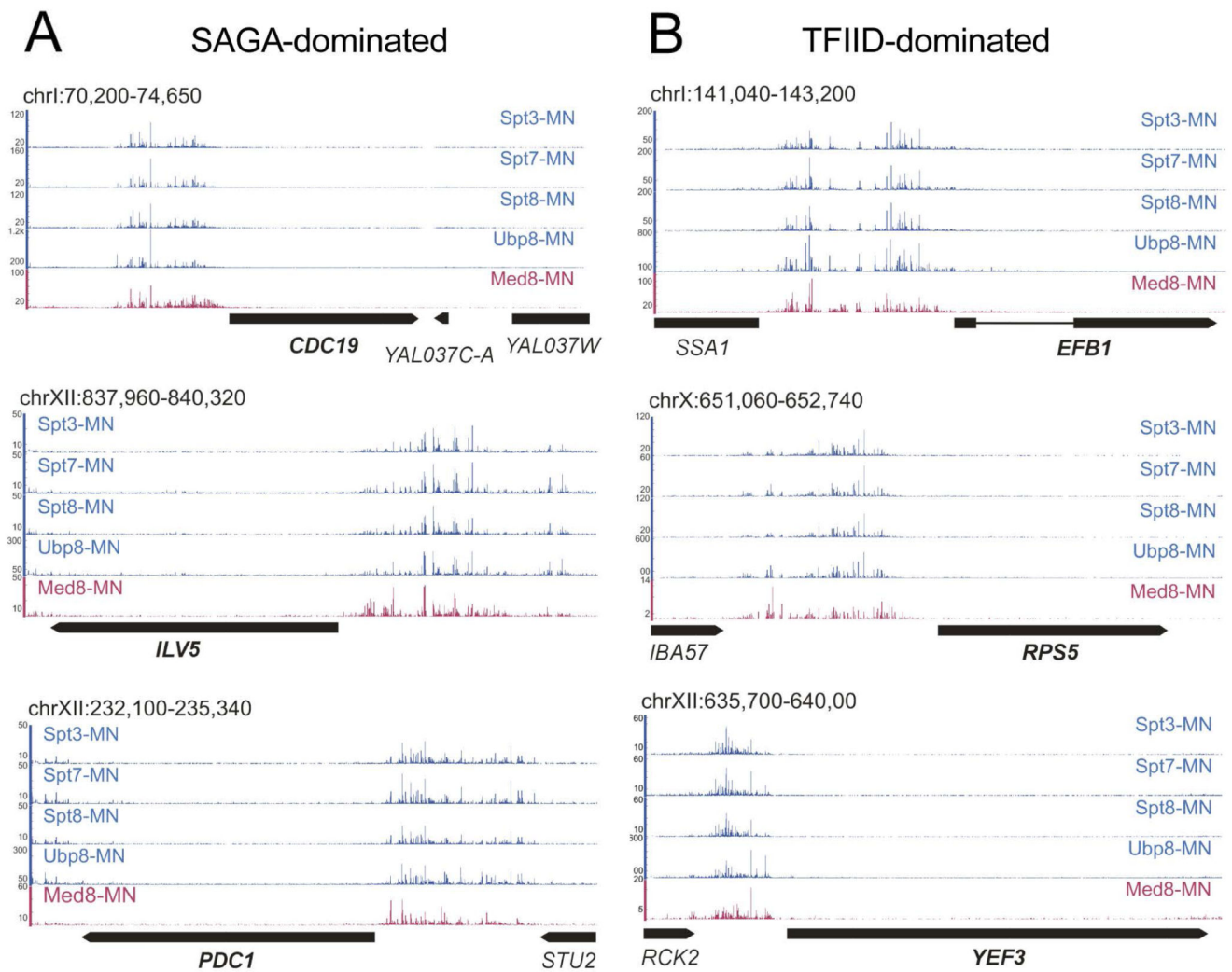
Figure 1. ChEC-seq profiling of SAGA specific subunits. Signal tracks showing cleavages induced by Spt3-MNase, Spt7-MNase, Spt8-MNase and Ubp8-MNase at (A) three representative SAGA-dominated genes ( CDC19 , ILV5 and PDC1 ) and (B) three TFIIID-dominated genes ( EFB1 , RPS5 and YEF3 ). Med8-MNase cleavage sites are shown as a reference for the coactivator Mediator binding at UASs (Grunberg et al., 2016). See also Figure S1.
