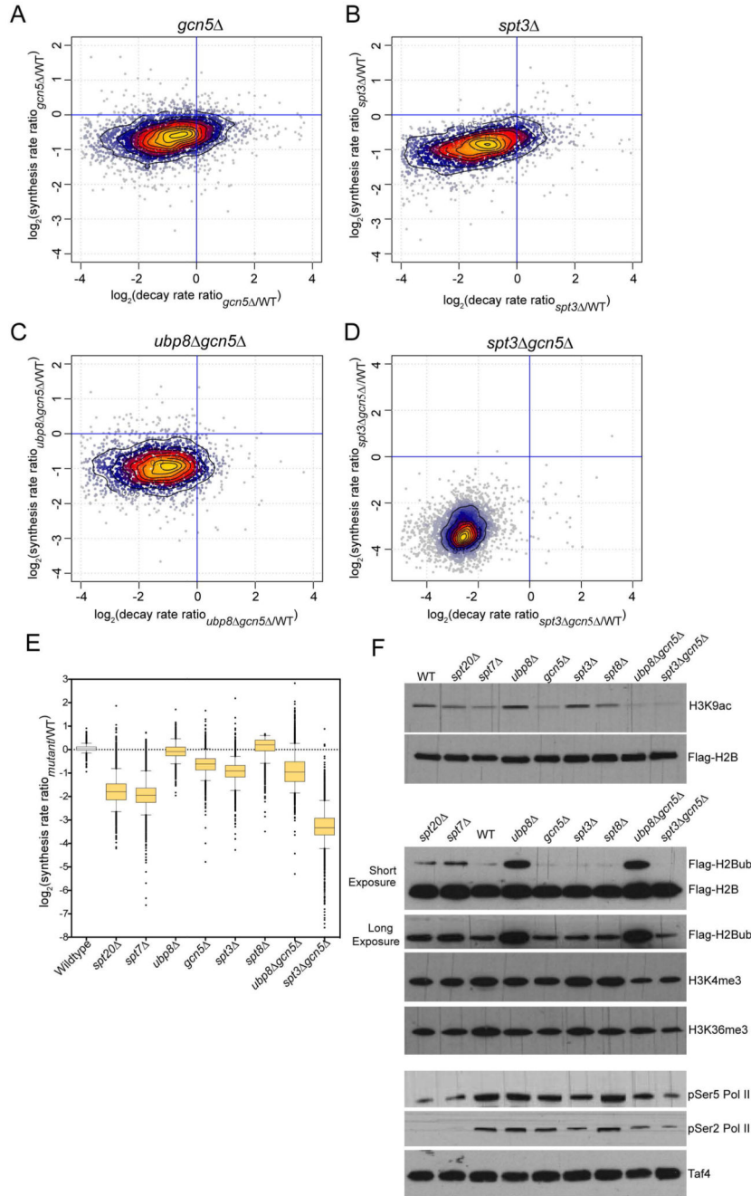
Figure 6. cDTA analyses of different SAGA subunit deletion strains. Synthesis rates and decay rates were determined for each S. cerevisiae gene in gcn5 (A), spt3 (B), ubp8 gcn5 (C) and spt3 gcn5 (D). Changes (calculated as the Log2 of the ratio between mutant and wild-type) in synthesis rates were plotted against changes in decay rates. (E) Box plots summarizing the extent of changes in mRNA synthesis for all the analyzed deletion strains. For each strain, cDTA data were obtained from at least two independent biological replicates. (F) Whole cell extracts from wild-type and the indicated deletion strains were revealed with the antibodies corresponding to histones marks regulated
