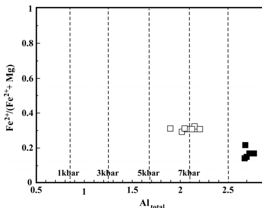
Figure 11. Plot of \text{Al}_{\text{total}} versus \text{Fe}^{2+}/(\text{Fe}^{2+} + \text{Mg}) for amphiboles from the hornblende xenoliths [Hammarstrom and Zen, 1968].
