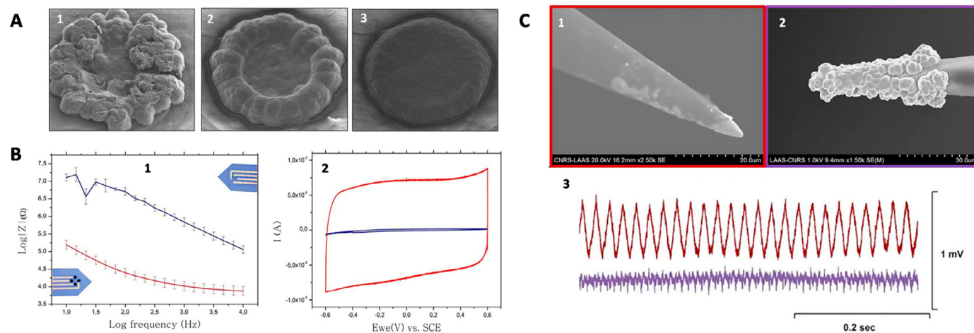
Fig. 3. Conductive polymers for neural interfaces. (A) SEM images of different morphologies of PEDOT:PSS layers related to different electrochemical deposition parameters. For 10 \mu\text{m} -diameter gold electrodes, the use of lower concentrations of monomer, lower upper vertex potentials and lower scan rates leads to a more homogeneous deposition. (B) Electrochemical characterization of parylene-based flexible neural microelectrodes with PEDOT coated surface. (A-1) Electrochemical mean impedance spectroscopy over a range of 10\text{--}10^4 Hz and related error bar and (A-2) charge storage capacity for the gold electrode (blue) and for the PEDOT-modified electrode (red) for a 10 \mu\text{m} diameter electrode in a NaCl 0.9% solution (Reprinted with a permission from Ref [104]). (C) SEM images of commercially available microelectrodes (alphaOmega, FHC): (B-1) uncoated electrode, (B-2) PEDOT:PSS-coated electrode (B-2). (B-3) Electric hum recorded in a mouse brain slice maintained in vitro by using commercial microelectrodes and nano-structured microelectrodes (Reprinted with a permission from Ref [104]).
