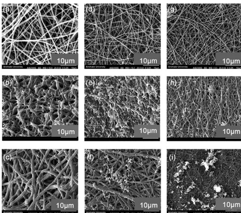
Fig. 12. Scanning electron micrographs ( \times 5,000 ) of (a) PVA fibers, (d) 80% PVA–20% chitosan fibers, (g) 60% PVA–40% chitosan fibers. (b), (e), and (h) Micrographs of crosslinked fibers, and (c), (f), and (i) micrographs of polypyrrole-coated PVA, 80% PVA–20% chitosan, and 60% PVA–40% chitosan fibers. The presence of electroactive agent resulted in a larger fibers and created a new surface structure (Reprinted with a permission from Ref [191]).
