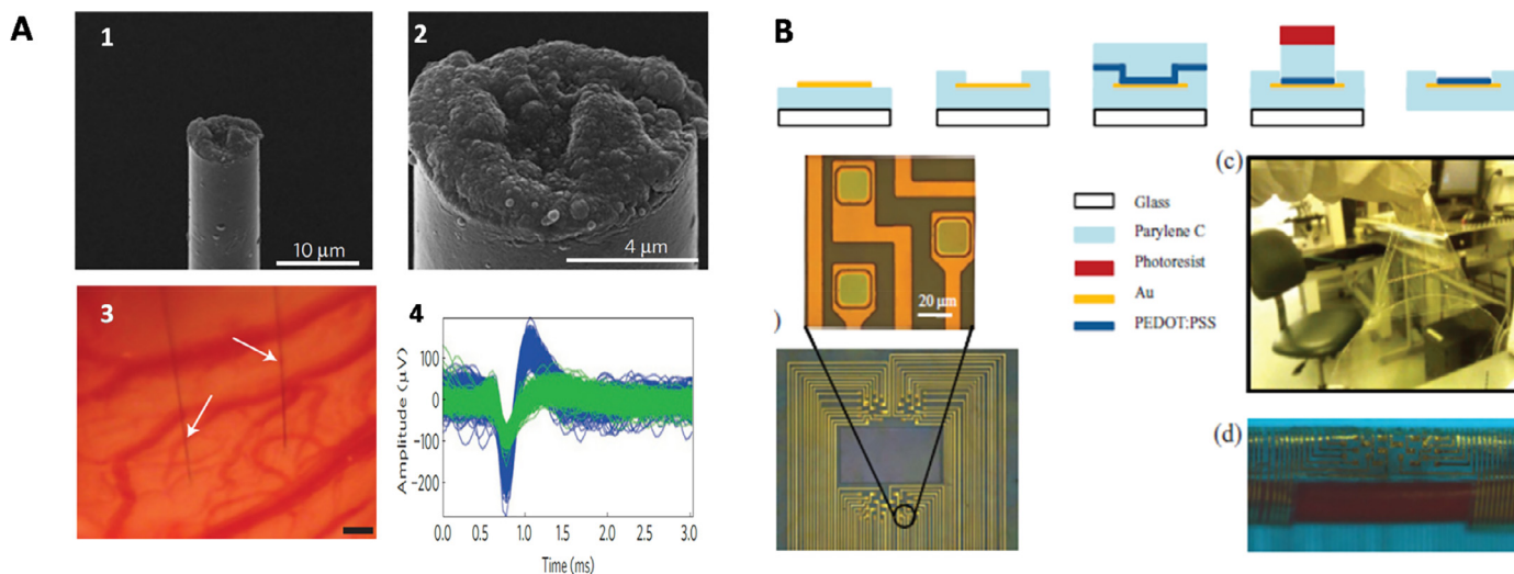
Fig. 4. (A) Ultrasmall carbon fiber microthread electrodes. (A-1) and (A-2) SEM images of the ultrasmall carbon fiber microelectrode ( \leq 7 \mu\text{m} in diameter) coated with PEDOT:PSS. (A-3) The microthread electrodes were implanted 1.6 mm deep into the cortex of adult male Sprague-Dawley rats. (A-4) Piled single-unit neural recordings over 3 min from a carbon fiber-coated PEDOT:PSS device (Reprinted with a permission from Ref [105]). (B) Conformable CP ECoG electrodes. Top: Schematic representation of the fabrication process indicating the cross-section of an electrode (not to scale). Down left: Microscopy images of the array showing the hole through which a silicon probe was inserted and a detailed view of three electrode. Down right: The electrode array is shown to support the weight of a quartz wafer (Reprinted with a permission from Ref [106]).
