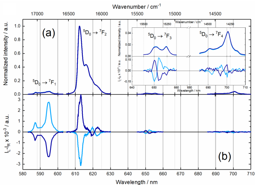
Figure 2. (a) Total emission and (b) CPL spectra measured in CH 2 Cl 2 solution under 280 nm (35714 cm -1 ) irradiation at room temperature for [( S,S,S )-2] (light blue line) and [( R,R,R )-2] (dark blue line). Inset: magnification of the range 640–710 nm (15625–14085 cm -1 ).
