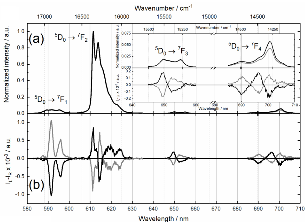
Figure 1. (a) Total emission and (b) CPL spectra measured in CH 2 Cl 2 solution under 280 nm (35714 cm -1 ) irradiation at room temperature for [( S )-1] (gray line) and [( R )-1] (black line). Inset: magnification of the range 640–710 nm (15625–14085 cm -1 ).
