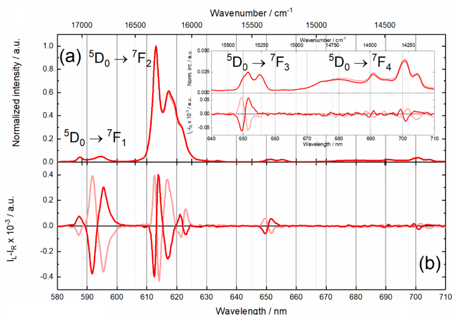
Figure 7. (a) Total emission and (b) CPL spectra measured in solid-state under 340 nm ( 29412\text{ cm}^{-1} ) irradiation at room temperature for [(S)\text{-}3]_n (light red line) and [(R)\text{-}3]_n (dark red line). Inset: magnification of the range 640–710 nm ( 15625\text{--}14085\text{ cm}^{-1} ).
