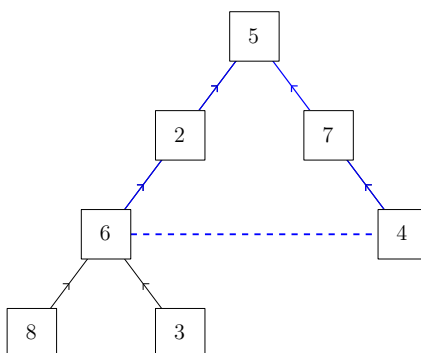
■ Figure 3 A set of oriented edges obtained by performing FindSet operations for the two nodes 6 and 4 of the same set. The dotted edge, which is not in the disjoint-set structure, illustrates how a cycle can be constructed from the structure.
