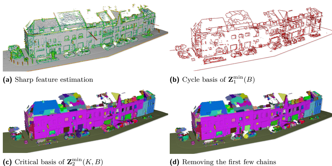
■ Figure 6 Example of reconstruction based on the construction of a critical basis. After choosing a threshold for the sharp feature estimation (a) and constructing an offset complex B , the basis of \mathbf{Z}_1^{\min}(B) forms a “wireframe” representation of the scene (b). The critical basis correctly reconstructs most parts of the scene (c). In this basis, the largest elements often correspond to the perceived holes of the original set of points (d).
