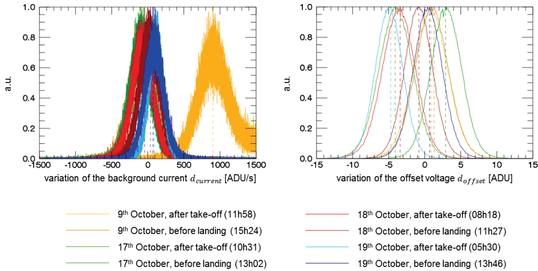
Figure 5. Normalized histogram of the difference between background measured in laboratory and background measured in flight Left: background current. Right: offset voltage
