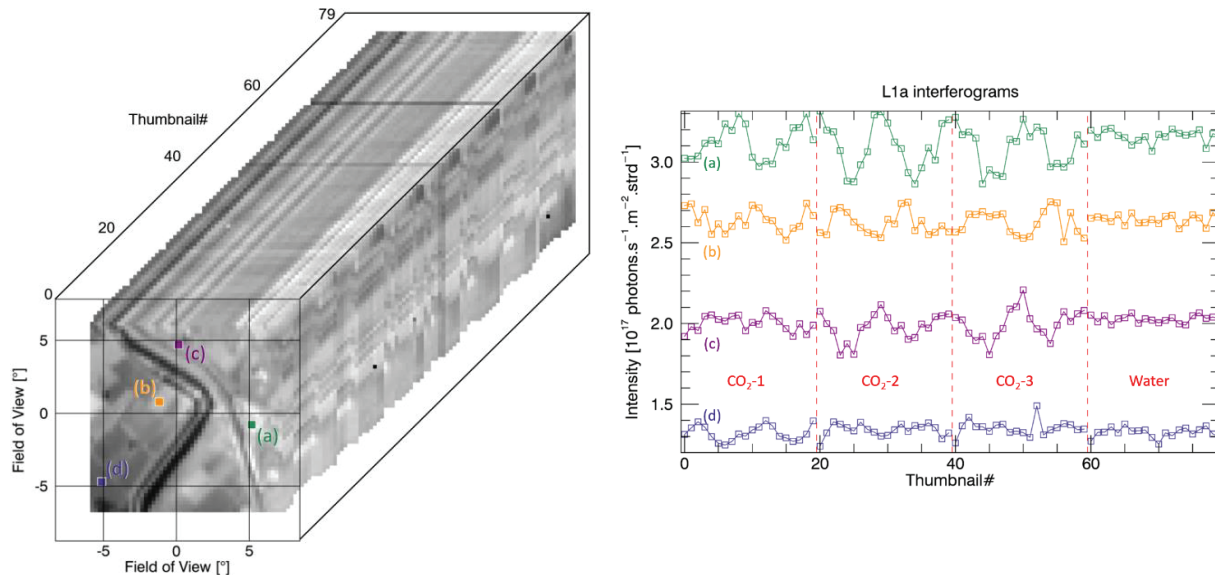
Figure 7. Left: Snapshot L1a cube of registered and radiometrically calibrated thumbnails. Right: some L1a interferograms extracted from this cube. Each curve's color corresponds to a colored point over the field of view of the left cube.
