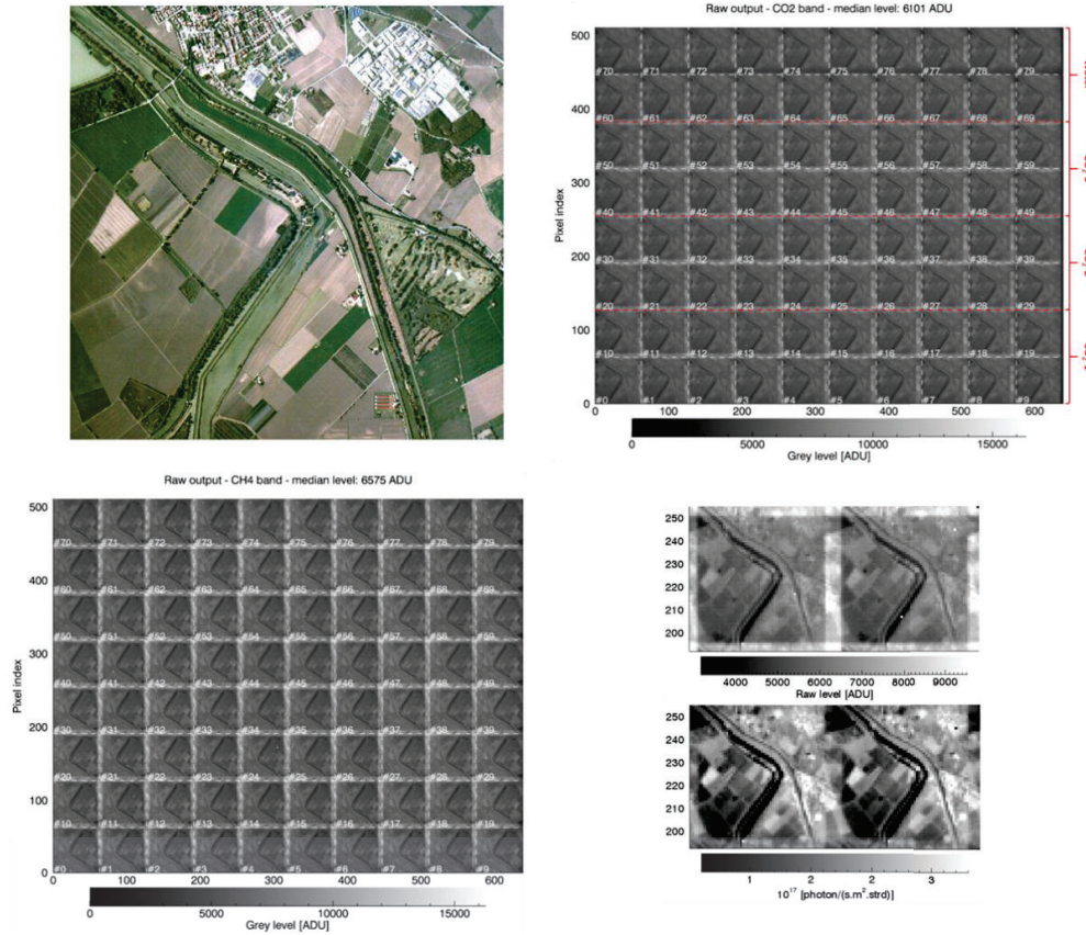
Figure 6. Top-left: context visible RGB picture from flight over Italy, October 17th 2020, between Adriatic sea and Modena, at 10 km of altitude. Top-right: CO 2 L0 raw frame. Bottom-left: CH 4 L0 raw frame. Superimposed thumbnail indexation and interferometric channels. CH 4 band has a single interferometric channel when CO 2 band has four. CH 4 camera is rotated by 180° compared to CO 2 . Picture is consequently reversed. Bottom-right: detail of the CO 2 raw image (top), corrected then expressed in radiometric unit (bottom).
