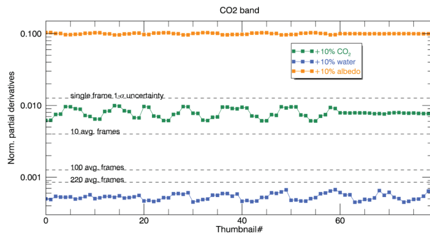
Figure 14. Comparison of the CO 2 band partial derivatives with 1-sigma noise level of snapshot interferogram, then L1b averaged time series. Maximum number of available frames in L1b level is ~220 at 10 km high with a framerate of 20 Hz.
