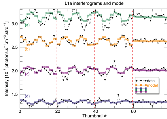
Figure 10. Some L1a interferograms in the field of view and associated models.
