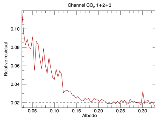
Figure 12. Relative residual plotted as a function of the estimated albedo, for the three CO 2 channels of the CO 2 band.
