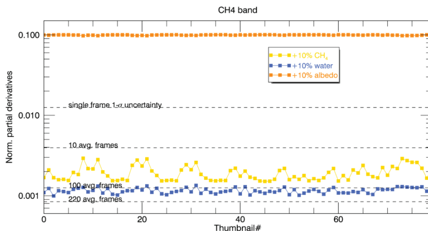
Figure 15. Comparison of the CH 4 band partial derivatives with 1-sigma noise level of snapshot interferogram, then L1b averaged time series. Maximum number of available frames in L1b level is ~220 at 10 km high with a framerate of 20 Hz.
