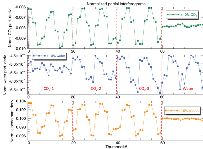
Figure 13. CO 2 band partial derivatives of L1a signal for CO 2 , water, and albedo, given a pixel on the center of the field of view and a nominal albedo of 0.22.
