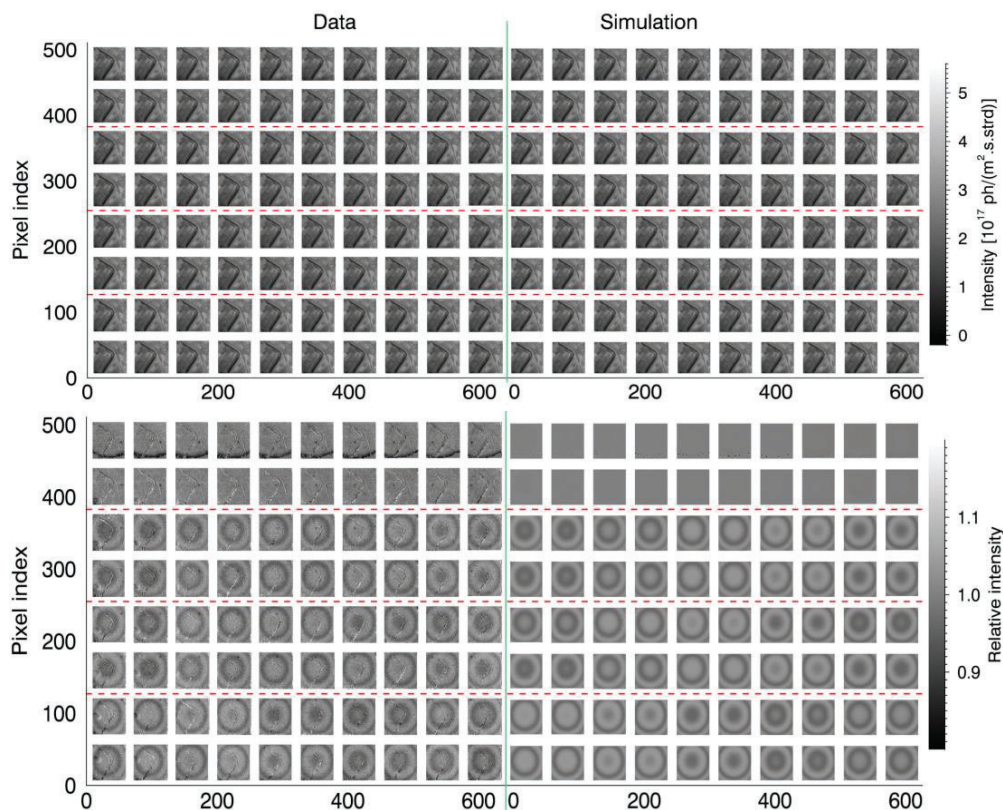
Figure 9. Top: Snapshot CO 2 processed frame extracted from data (Left) compared with model (right). Bottom: a normalization by panchromatic picture make apparent interferometric signature of the atmospheric absorption. Radiometric model shows a well adequacy with data.
