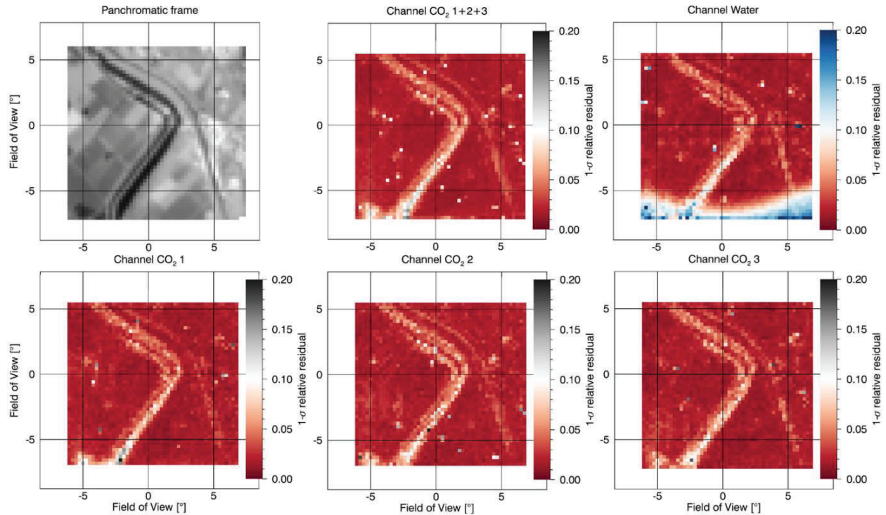
Figure 11. Relative residual shown over the field of view, over the different interferometric channels of the CO 2 band.
