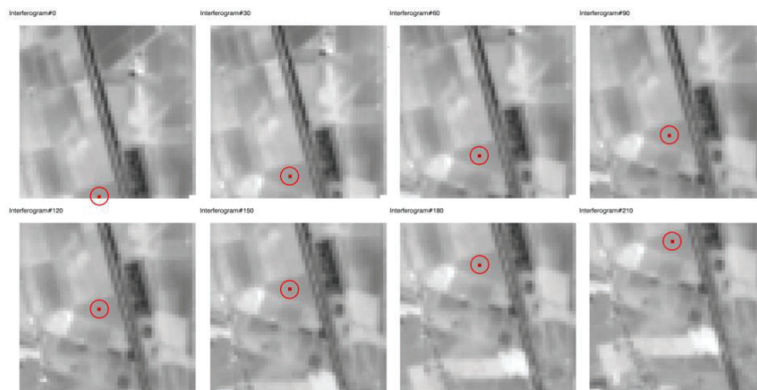
Figure 8. Time sequence of acquisitions over the CO 2 band, showing successive panchromatic CO 2 images. Panchromatic frame is defined as the averaged of all the thumbnails for each band. L1b time series of interferograms are extracted as an example for the surrounded red point at ground from the time sequence of L1a cube.
