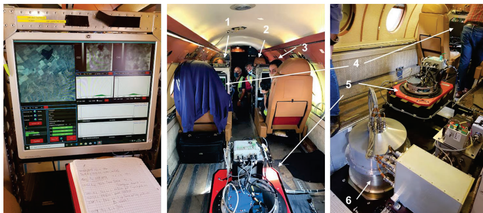
Figure 3. Left: NanoCarb user interface, seen from the NanoCarb operator seat. The image on the left is the visible image, while the two black and white images on the right are one thumbnail from the CO 2 and the CH 4 cameras. Middle and right: inside of the F20 1: Safire operator, 2: NanoCarb operator, 3: NanoCarb observer, 4: Spex operator, 5: GSM with the NanoCarb cameras, 6: SpexAirborne.
