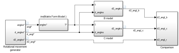
Fig. 13. Simulation schema; (B) model = Eq.23, (C) model = Eq.24, angles^* = \varepsilon^* , dangles^* = \dot{\varepsilon}^* , d2angles^* = \ddot{\varepsilon}^*
