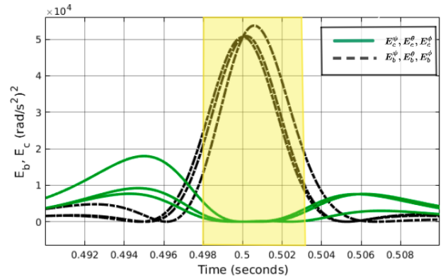
Fig. 14. E_c and E_b represent resp the models Eq.24 -23 errors.
