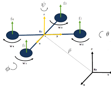
Fig. 7. Quadrotor model in the space
