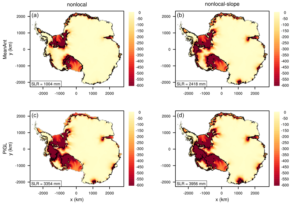
Figure 8. Same as Fig. 7, but with thermal forcing increasing by 2 °C between 1950 and 2100 and held fixed thereafter. In the nonlocal runs (a, c), black lines are absent at the present-day calving fronts of several ice shelves, indicating shelf collapse.
