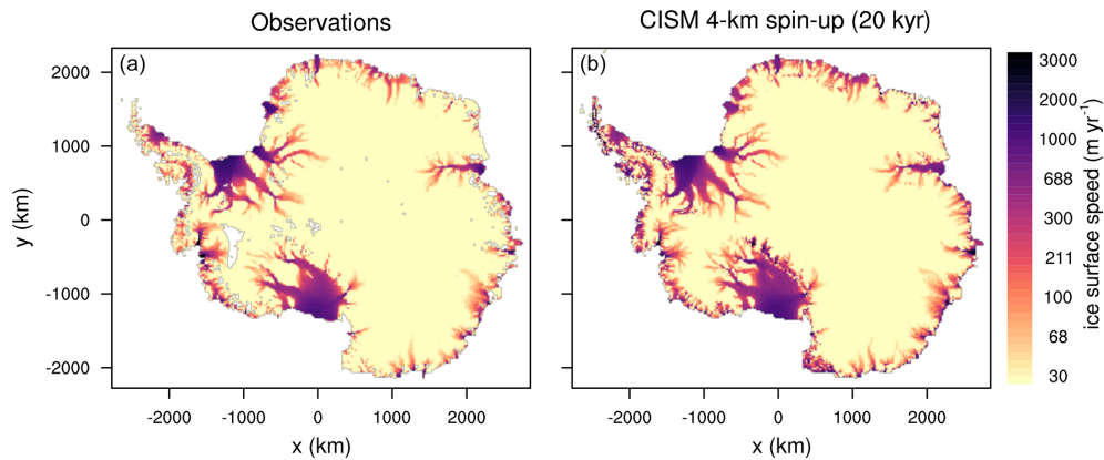
Figure 4. Antarctic ice surface speed ( \text{m yr}^{-1} , log scale) from (a) observations (Rignot et al., 2011) and (b) the end of a 20 kyr CISM spin-up at 4 km resolution using the nonlocal-MeanAnt melt parameterization and calibration.
