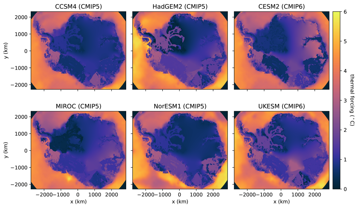
Figure 9. Ocean thermal forcing (°C) at z = -510 m, averaged over 2081–2100, for the four CMIP5 models and two CMIP6 models used in ocean-forced projection experiments. Thermal forcing is used to compute basal melt rates in grid cells with floating ice.
