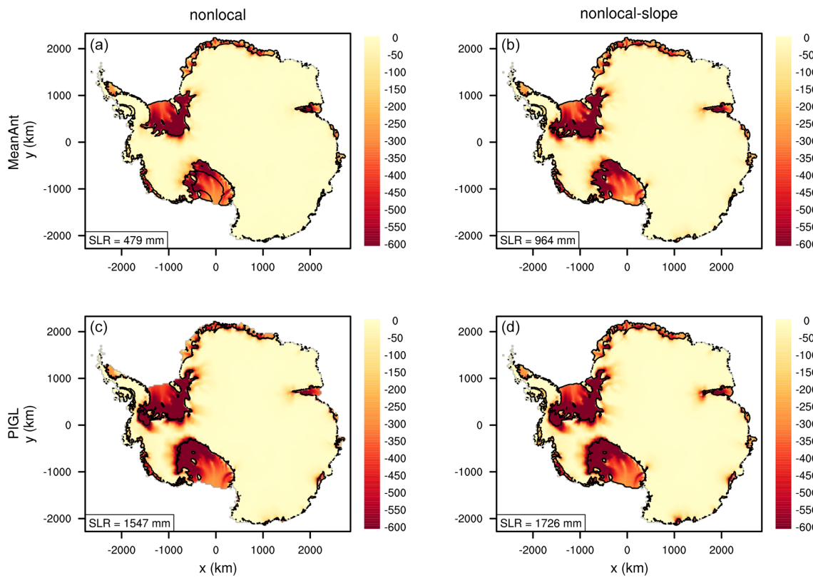
Figure 7. Difference in ice thickness (m) between the years 2500 and 1950 in experiments with idealized ocean forcing. Starting from the spin-up state, thermal forcing increases by 1^{\circ}\text{C} between 1950 and 2100 and is held fixed thereafter. The two columns correspond to the nonlocal and nonlocal-slope melt parameterizations, and the two rows to the MeanAnt and PIGL calibrations. Black lines show boundaries of floating ice at the end of each run. In the nonlocal-PIGL run (c), black lines at the present-day calving fronts of several large ice shelves are absent, indicating shelf collapse. In the nonlocal-MeanAnt run (a), the Ross Ice Shelf partly collapses. Boxes in the lower left of each panel show the SLR contribution from the loss of grounded ice.
