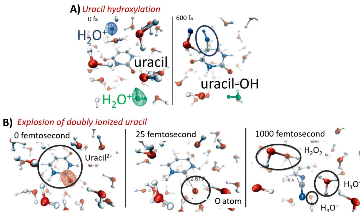
Figure 8: Hydroxylation of the solvated uracil by H 2 O + formed in its solvation shell (Top) and Coulomb explosion after double ionization. Adapted with permission from ((116)).
