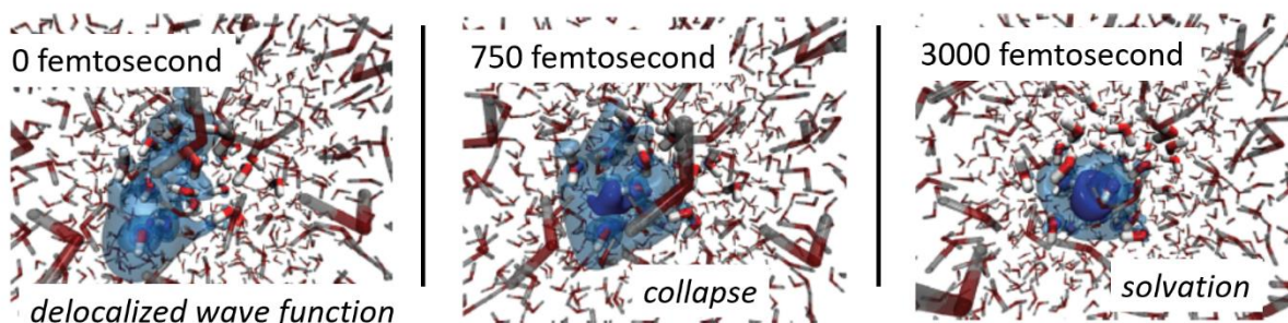
Figure 7: electron wave function collapse and electron solvation after initial excitation. Adapted with permission from Ref. (105).
