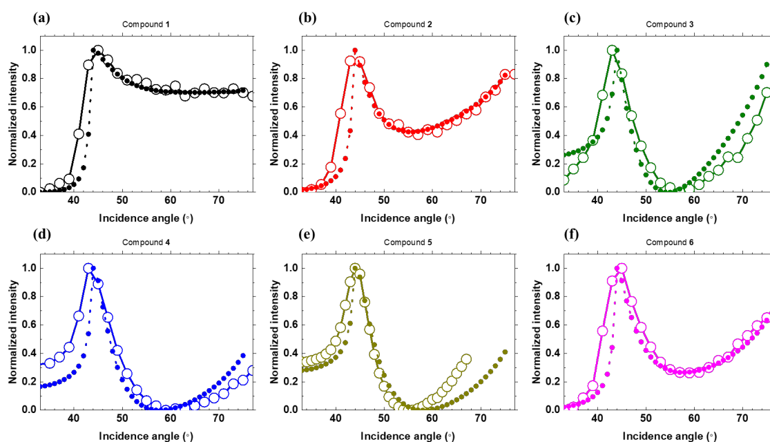
Figure 8. Experimental (open circle) and FDTD simulated (closed circle) ATR spectra for six Curc series.
