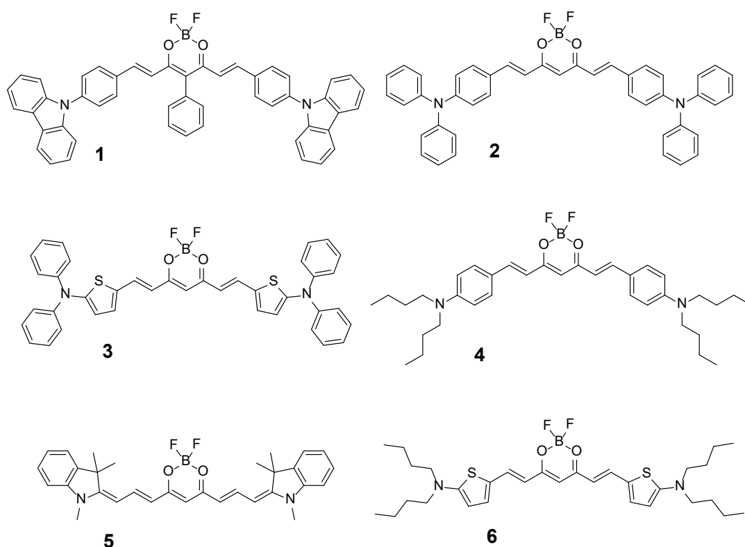
Figure 1. Molecular structure of compound 1 , 2 , 3 , 4 , 5 , and 6 . Compound 1 is curcuminoid – carbazol (Curc-CBz), compound 2 is Curcuminoid -triphenylamine (Curc-TPA), compound 3 is Curcuminoid-Thiophene(Curc-ThiopPh), compound 4 is Curcuminoid-dibutylAmine (Curc-PhNBu 2 ), compound 5 is Curcuminoid-Indol (Curc-Indol), and compound 6 is Curcuminoid-Thiophene dibutylamine (Curc-ThiopBu 2 ).
