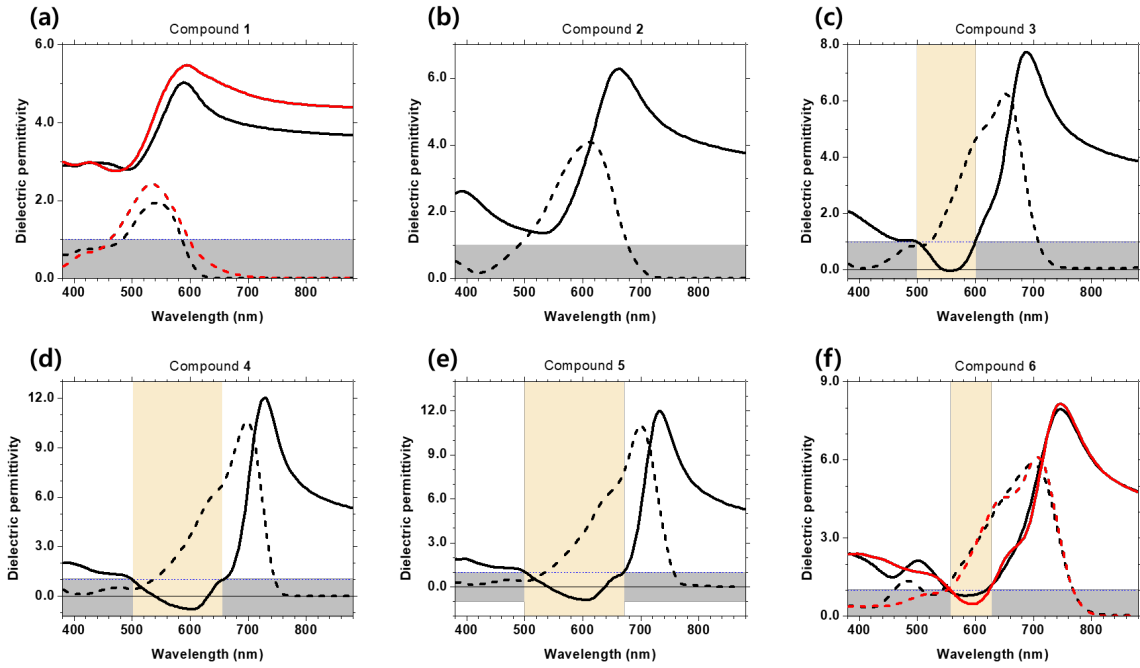
Figure 5 Dielectric permittivity spectra of the six Curc series are plotted in increasing order of donor strength from (a) to (f). Solid (dashed) black and red curves refer to the real (imaginary) part of dielectric permittivity. In (a) and (f) black and red curves correspond to parallel and perpendicular components of dielectric permittivity, respectively.
