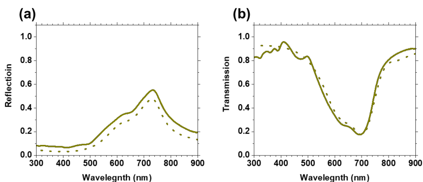
Figure 7. Experimental (solid curve) and FDTD simulated (dashed curve) reflection (a) and transmission (b) spectra of film 5 are compared.
