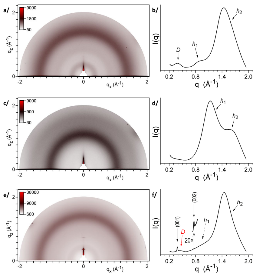
Figure S5 | GIWAXS pattern (a/, c/ and e/) and the corresponding radial profile (b/, d/ and f/) of compound 4 (a/ and b/), 5 (c/ and d/) and 6 (e/ and f/).
