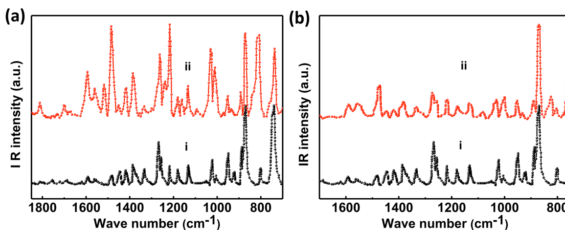
Fig. 10: (a) PM-IRRAS spectra of DNTT layer formed on FBPS-grafted oxidized (by RCA (1/1/16000)) KBr pellet (i) and Cu surface (ii); (b) PM-IRRAS spectra of DNTT layer formed on BPS-grafted oxidized (by RCA (1/1/16000)) KBr pellet (i) and Cu surface (ii).
