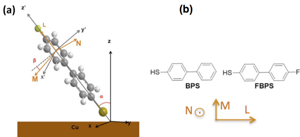
Fig. 1: (a) Orientation of transition dipolar moment associated with the three possible directions of vibration polarization of FBPS; (b) Chemical structures of BPS and of FBPS.
