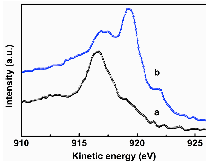
Fig. 7: Cu L3M4, 5M4, 5 spectra of (a) Cu/RCA (1/1/16000)/FBPS; b) FBPS adsorbed on Cu treated by RCA solution and then by citric acid.
