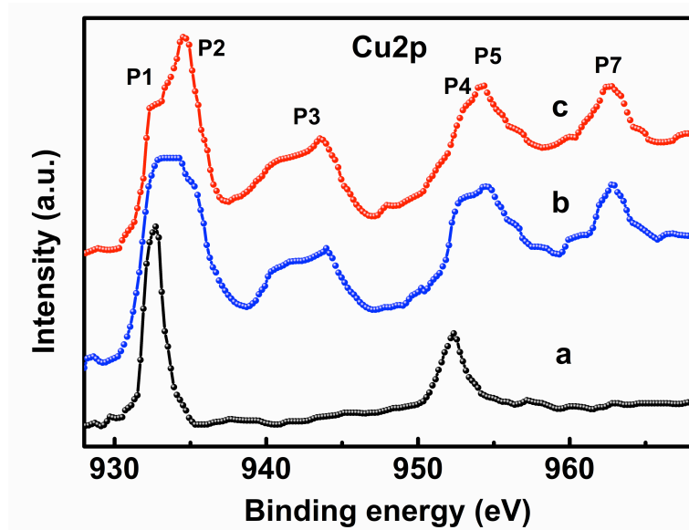
Fig. 6: XPS \text{Cu}2p spectra at different Cu treatment conditions: (a) \text{Cu/RCA (1/1/16000)/FBPS} ; (b) \text{Cu/RCA (1/1/16000)} ; (c) \text{Cu/RCA (1/1/16000)/BPS} .
