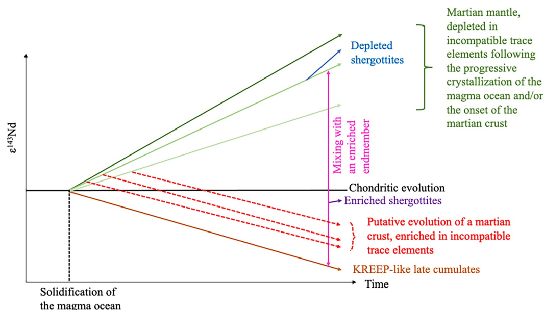
Figure 16. Schematic geodynamical evolution of the martian interior : Radiogenic ingrowth of ^{143}\text{Nd}/^{144}\text{Nd} depends on the variation in Sm/Nd in the reservoirs. The progressive solidification of the magma ocean resulted in several depleted reservoirs (in green) and ended up with enriched late cumulates (in brown), after Debaille et al. (2007). From the depleted martian mantle, a crust has been extracted, that is enriched in incompatible trace elements, as observed in NWA 7034 (Arnytag et al., 2018). Depleted shergottites (in blue) directly sample a depleted reservoir while the enriched shergottites (in violet) represent a mixture (in pink) between depleted and enriched reservoirs.
