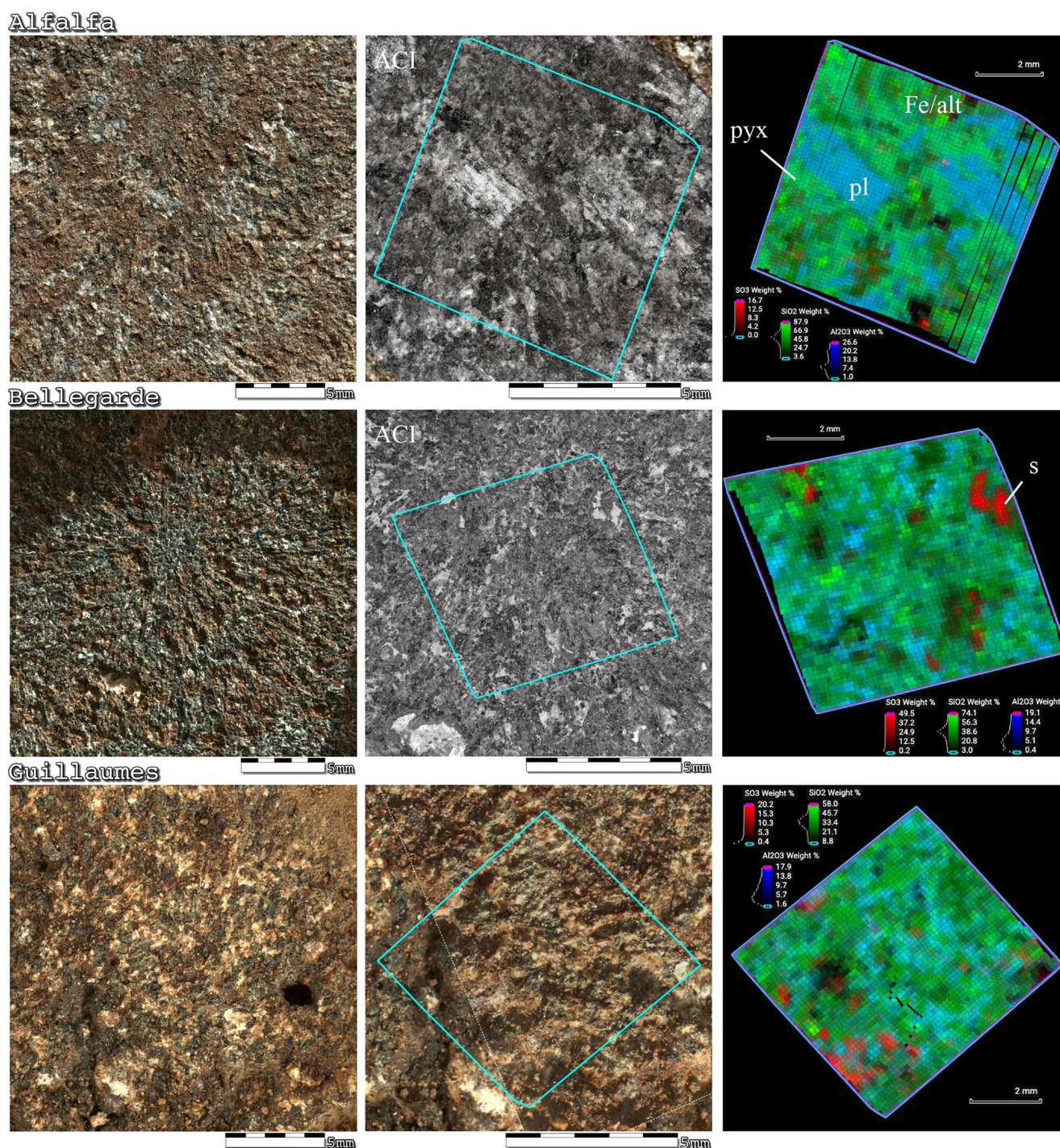
Figure 13. Close up observations of Máz abrasion sites by WATSON (~4 cm standoff), Autofocus and Context imager (ACI), and PIXL: Compositional X-ray map of SO 3 (red), SiO 2 (green), and Al 2 O 3 (blue) concentrations, generally correspond to primary pyroxene (pyx) = light green, plagioclase (pl) = blue, and Fe-silicate/olivine (Fe/alt) = green and secondary sulfate (s) = red, respectively (see text and Figures S12–S16, Table S1 in Supporting Information S1 for additional information). Colorized ACI used to improve image clarity for Guillaumes because of lighting conditions.
