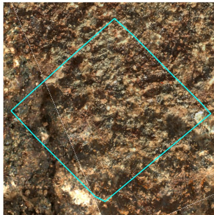
Figure 13. Close up observations of M á az abrasion sites by WATSON (~4 cm standoff), Autofocus and Context imager (ACI), and PIXL: Compositional X-ray map of SO 3 (red), SiO 2 (green), and Al 2 O 3 (blue) concentrations, generally correspond to primary pyroxene (pyx) = light green, plagioclase (pl) = blue, and Fe-silicate/olivine (Fe/alt) = green and secondary sulfate (s) = red, respectively (see text and Figures S12–S16, Table S1 in Supporting Information S1 for additional information). Colorized ACI used to improve image clarity for Guillaumes because of lighting conditions.
