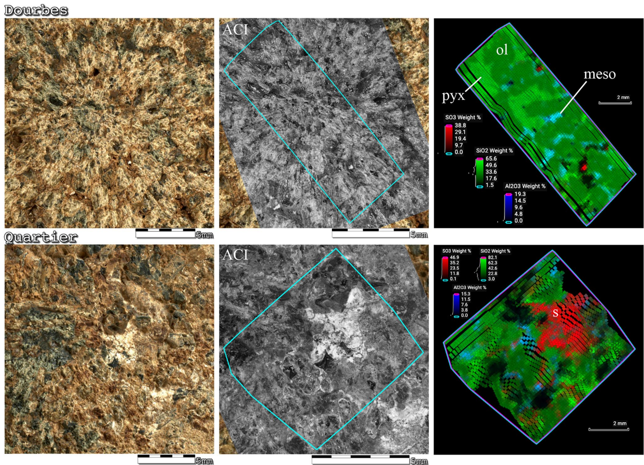
Figure 9. Close up observations of Séitah abrasion sites by WATSON (~4 cm standoff), Autofocus and Context imager, and PIXL: Compositional X-ray map of \text{SO}_3 (red), \text{SiO}_2 (green), and \text{Al}_2\text{O}_3 (blue) concentrations, generally correspond to primary olivine (ol) = dark green and pyroxene (pyx) = light green, compositionally evolved intercumulus mesostasis (meso) = blue and secondary sulfate (s) = red, respectively (see text and Figures S12–S16, Table S1 in Supporting Information S1 for additional information).
