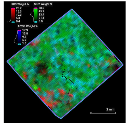
Figure 13. Close up observations of M á az abrasion sites by WATSON (~4 cm standoff), Autofocus and Context imager (ACI), and PIXL: Compositional X-ray map of SO 3 (red), SiO 2 (green), and Al 2 O 3 (blue) concentrations, generally correspond to primary pyroxene (pyx) = light green, plagioclase (pl) = blue, and Fe-silicate/olivine (Fe/alt) = green and secondary sulfate (s) = red, respectively (see text and Figures S12–S16, Table S1 in Supporting Information S1 for additional information). Colorized ACI used to improve image clarity for Guillaumes because of lighting conditions.
