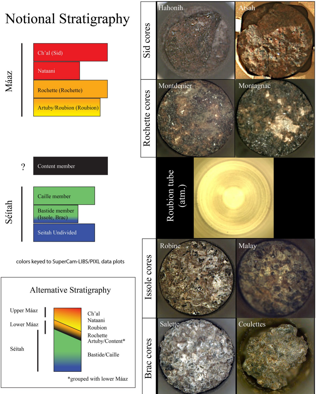
Figure 2. Samples from Jezero Crater floor collected by Perseverance: CacheCam images of rock sample cores from Séítah and Máaz units and tube of atmospheric gas prior to sealing. Core diameters are approximately 1.3 cm. Notional and alternative crater floor stratigraphic relationships of sampled units shown for reference (see Crumpler et al. (2023) and B. Horgan et al. (2022)).
