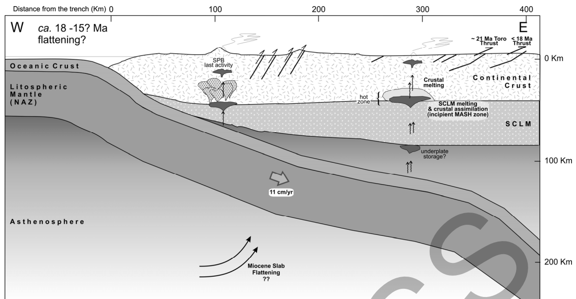
Figure 19: Schematic W-E section at ca. 51°S, illustrating a possible flat slab subduction scenario prior to the Chile Rise collision at ca. 18-16 Ma, for the alkaline magma generation of the Monte Balmaceda intrusive complex. Thrusting in the foreland region, pre- and post-dating the 18 Ma, is shown (from Fosdick et al. , 2011). Subducted slab geometry is inspired in the present flat slab subduction zone at 27-33°S in South America (e.g. Kay and Mpodozis, 2002; Deshayes et al. , 2008). The "Hot Zone" is following Annen et al. (2006). SPB: South Patagonian batholith, SCLM: Sub-Continental Lithospheric Mantle. NAZ: Nazca plate. 11cm/a: average convergence rate between Nazca and South American plates, from Pardo-Casas and Molnar (1987), Somoza (1998) and Breitsprecher and Thorkelson (2009) data.
