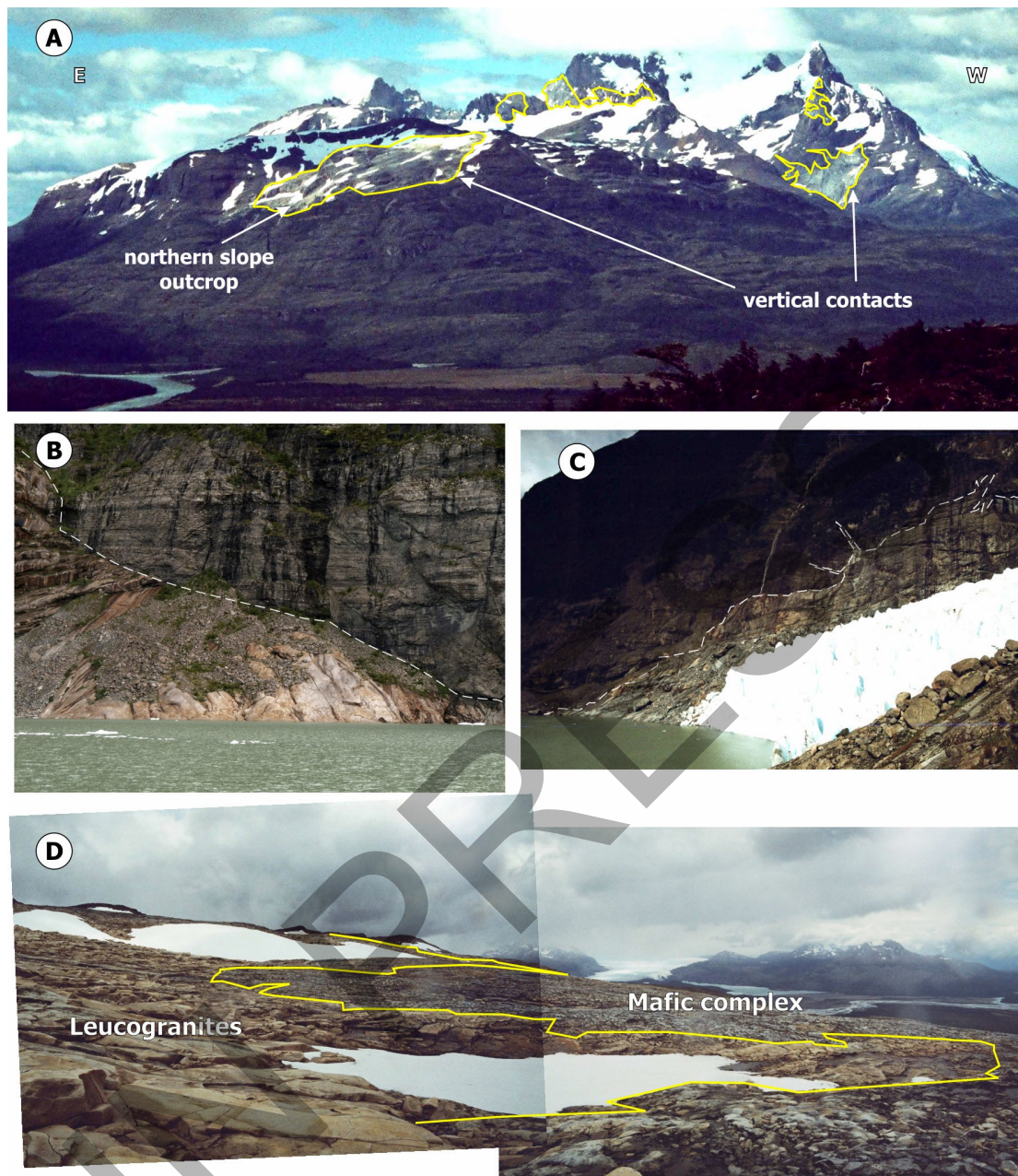
Figure 8: Field photographs from the Monte Balmaceda intrusive complex, southern area. A. Panoramic view of the northern face of the Monte Balmaceda. Some of the disconnected outcrops of intrusive rocks are shown highlighted by yellow borders. B. Discordant intrusive contacts with sub-horizontal layered sedimentary rocks. C. Intrusive contact showing some "stepping", a common feature in the Glaciar Serrano area. D. Zig-zag contact between the Leucogranites and the Balmaceda Mafic Complex, the outcrop is in the Monte Balmaceda northern face. This pattern is caused by the subhorizontal contact between these units, with the mafic unit below the felsic one.
