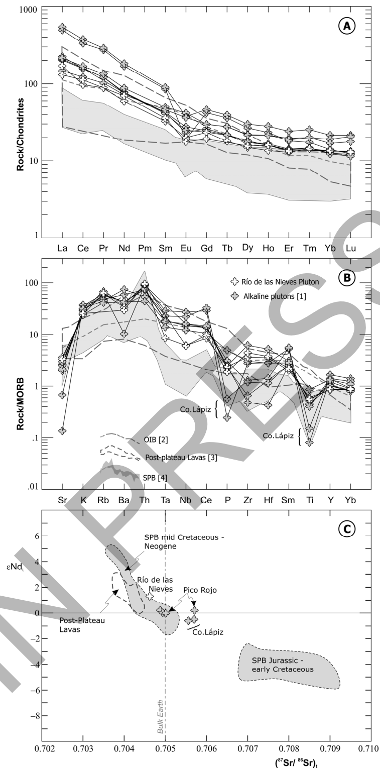
Figure 14: Trace elements and isotopic composition diagrams for the Pliocene northern area plutons. A. REE diagrams normalized to chondrite (Nakamura, 1974). B. Spider diagrams normalized to MORB (Pearce, 1983). C. \epsilon Nd_t vs. (^{87}Sr/^{86}Sr)_i . References: 1: Espinoza et al. (2008); 2: Sun and McDonough, (1989); 3: Gorrington and Kay (2001); 4: Hervé et al. (2007).
