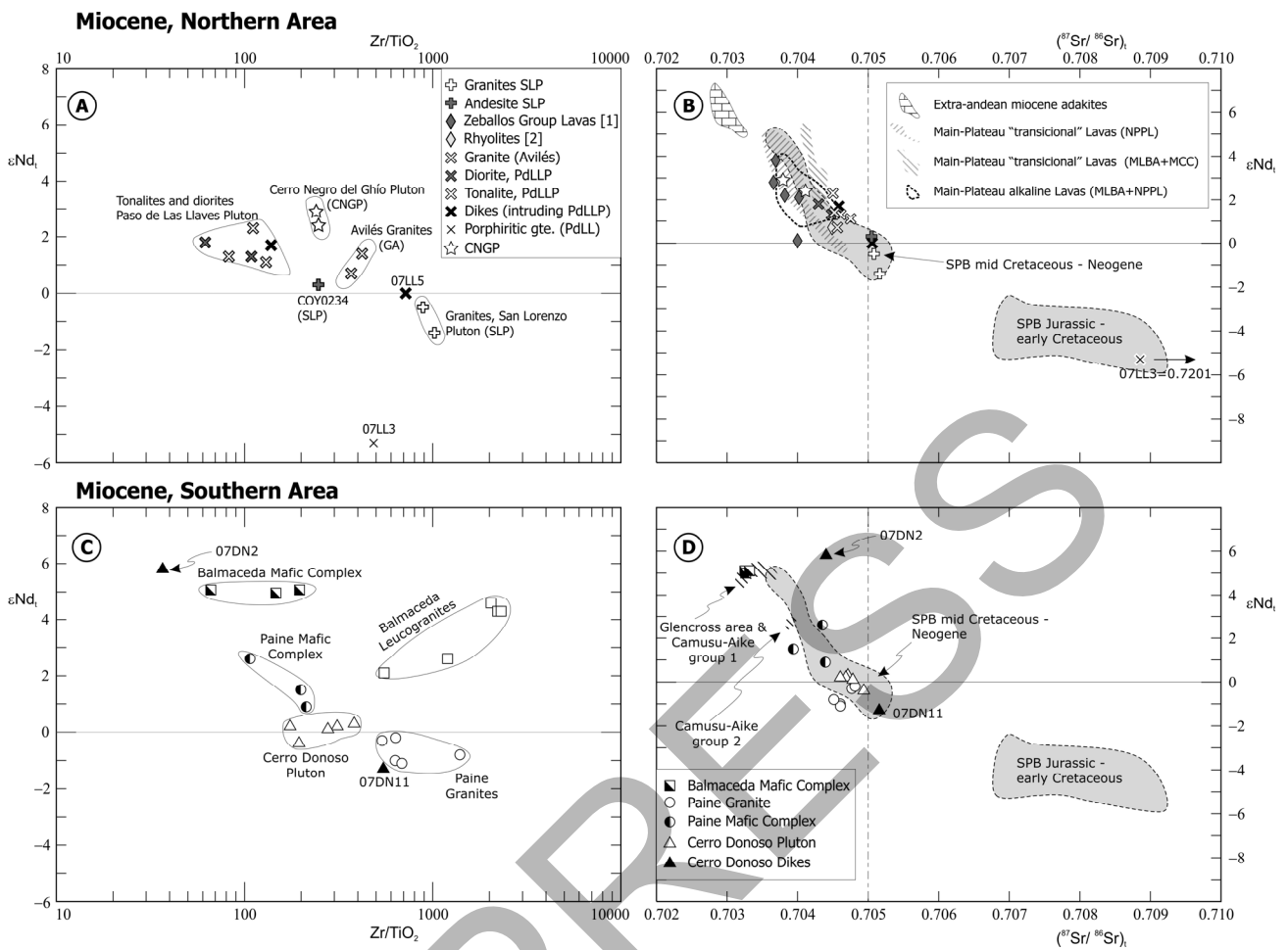
Figure 13: Isotopic composition diagrams for Miocene plutons from the northern and southern areas. A. \epsilon\text{Nd}_t vs \text{Zr}/\text{TiO}_2 ratio for plutons from the northern area. 1: Zeballos Group Lavas, Espinoza et al. (2010); 2: Miocene rhyolites, Espinoza et al. (2005). B. \epsilon\text{Nd}_t vs (^{87}\text{Sr}/^{86}\text{Sr})_i ratio for plutons from the northern area, with bulk Earth divisions at present time. Data plotted for comparison: Extra-andean adakites (Ramos et al. , 2004); Miocene "transicional" and alkaline lavas (Gorring and Kay, 2001; Espinoza et al. , 2005; Guivel et al. , 2006). C. \epsilon\text{Nd}_t vs \text{Zr}/\text{TiO}_2 ratio for plutons from the southern area. D. \epsilon\text{Nd}_t vs (^{87}\text{Sr}/^{86}\text{Sr})_i ratio for plutons from the southern area. Data is compared with the isotopic composition of the Glencross Area and Camusú-Aike volcanic fields (D'Orazio et al. , 2001 and 2005 respectively). In B and D, SPB data is from Hervé et al. (2007).
