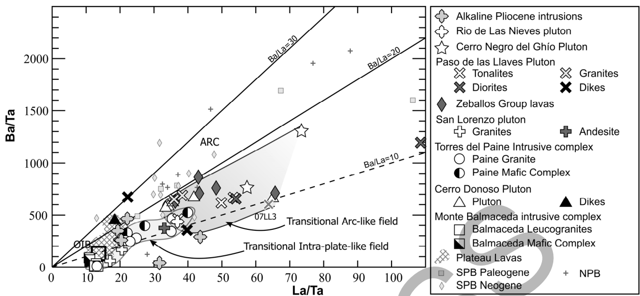
Figure 16: Ba/Ta vs La/Ta diagram, after Kay and Mpodozis (2002) for plutons from the northern and southern areas. Calc-alkaline arc signature is represented by the North and South Patagonian batholith samples (NPB, SPB), most of them with La/Ta >25 and Ba/La >20 (NPB and SPB data from Pankhurst et al. (1999) and Hervé et al. (2007), respectively). The plateau lavas, and OIB signatures, are well constrained, mostly with La/Ta between 10 and 20. In general terms, the plutonic samples from this study show two intermediate patterns, both with Ba/La <20 (lower than calc-alkaline arc-like) but with La/Ta either close to the arc, or to the intra-plate signatures. The Zeballos Group data is from Espinoza et al. (2010); References for the Plateau Lavas data as in Fig. 14.
