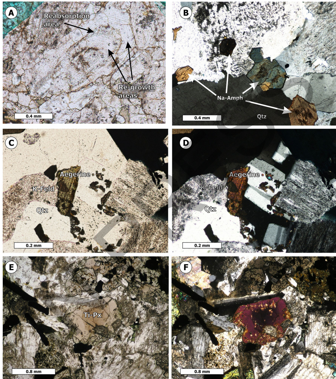
Figure 7: Micro-photographs. A. Plagioclase with several growth stages, plane light, from the granite in Cerro Donoso pluton. B. Sodic amphiboles in the leucogranite facies, polarized light. C. Aegerine pyroxene in the leucogranites, plane light. D. Idem C , polarized light. E. Titanium-rich augite in the alkaline gabbro. F. Idem E , polarized light. B to F are from the Monte Balmaceda intrusive complex.
