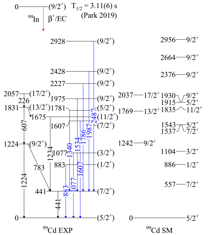
FIG. 4. Level schemes of ^{99}\text{Cd} from the \beta\gamma spectroscopy of ^{99}\text{In} . The half-life of ^{99}\text{In} was determined in a previous work (Park 2019 [23]). The energies of the states and the transitions are in keV. The states which are linked by black arrows were previously assigned in Ref. [8]. New \gamma rays which were placed in the level scheme of ^{99}\text{Cd} are drawn as blue arrows. For the SM results, only the most relevant states for comparison with the proposed experimental level scheme are shown.
