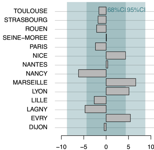
Fig. 14. Intercept random effects for Model 1 during the second wave of the epidemic for 14 WWTPs. A positive (resp. negative) intercept effect means the WWI should be lowered (resp. increased) in order to reflect the epidemic state in the same way that the incidence rate does. The deviations at most shortly exceed 5 units of the WWI: for Nancy , Lagny-sur-Marne (negative intercept effect), Marseille , Lyon , and Evry (positive intercept effects) which is acceptable, the WWI typically ranging from -50 to 150. The WWTP of Paris Seine-Amont was used for the comparison with the Grand Paris incidence rate.
