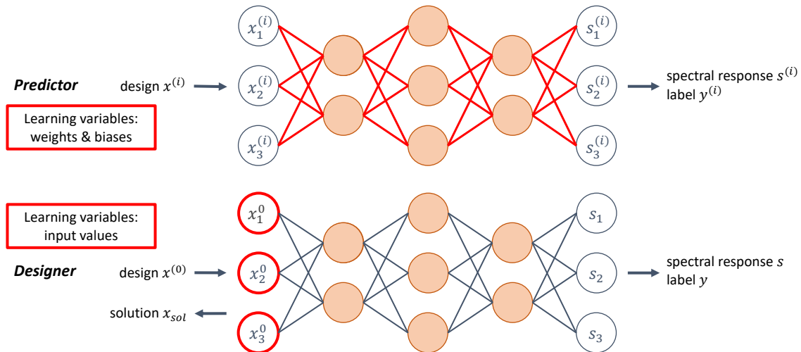
Fig. 1. predictor & designer design framework. The predictor is trained to predict spectral responses of given designs. The designer is a frozen copy of the predictor (fixed weights and biases); the training only modifies the input values.
