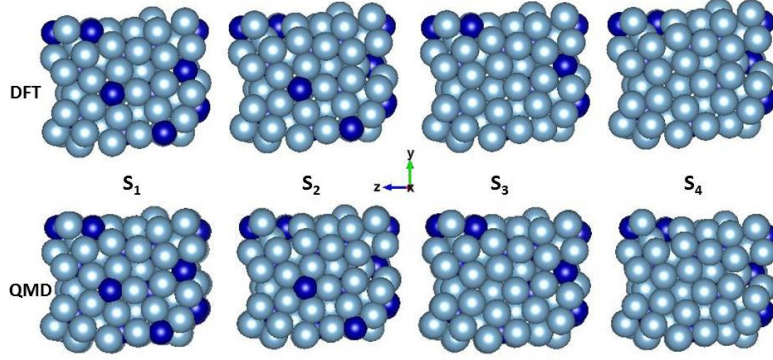
Figure 6: Model structures of P_2 -termination (almost complete). The models numbered from 1 to 4 are the denser ones for this surface. Dark blue and light blue balls correspond respectively to Co and Al atoms. The upper images correspond to the structures optimized with DFT and the lower ones to the same structures further relaxed by classical QMD.
