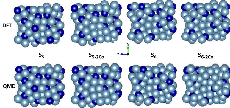
Figure 7: Incomplete surface terminations for the P_2 layer. Dark blue and light blue balls correspond to Co and Al atoms respectively. The upper images correspond to the structures optimized by DFT and the lower ones to the same structures further relaxed by classical QMD.
