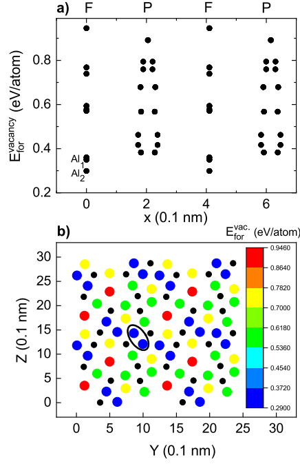
Figure 5: Al vacancy formation energies per site in bulk o- \text{Al}_{13}\text{Co}_4 . a) Representation along the direction perpendicular to the alternating F - and P - planes. b) Mapping of the Al vacancy formation energies in one F -plane. The scale on the right hand side of the graph illustrates the used color code, going from the smallest values of energies (blue) to the largest ones (red). The black ellipse contains two circles corresponding to \text{Al}_2 -type sites. The positions of Co atoms have been marked by small black circles for a better visualization of the structure.
