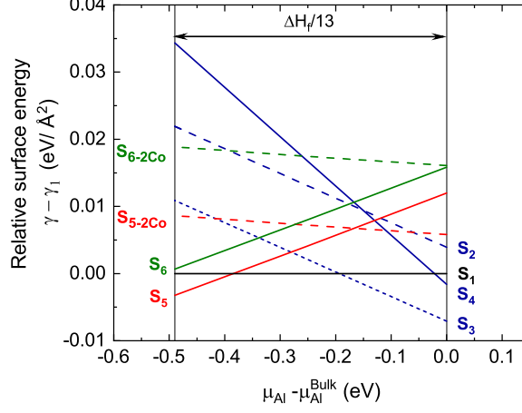
Figure 8: Relative surface energy vs the chemical potential \mu_{Al} - \mu_{Al}^{bulk} for the different models of Figures 6 and 7.
