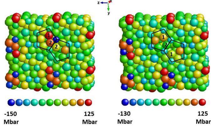
Figure 4: Optimized bulk atomic structures of \text{o-Al}_{13}\text{Co}_4 (crystallite of 815 atoms) obtained by QMD after removing one \text{Al}_1 -type atom from the ideal structure (left image) or one \text{Al}_2 -type atom (right image). Large and small balls correspond to Al and Co atoms respectively. The bottom pictures illustrate the used color code in the atomic structures, going from the maximal value of pressure (red) to the minimal one (blue).
