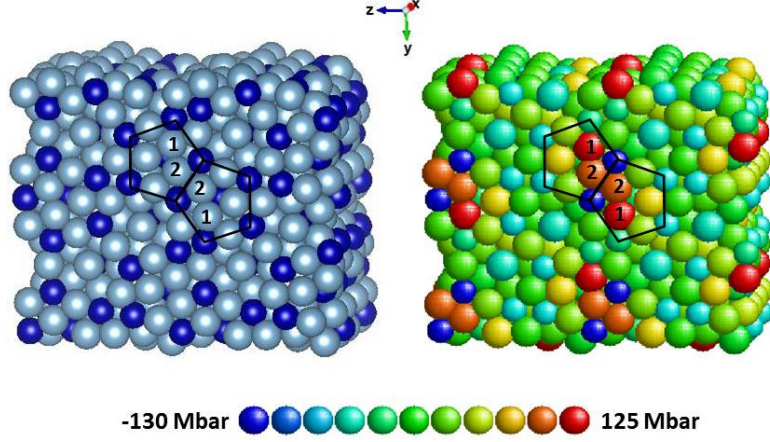
Figure 3: Left image : bulk atomic structure of \text{o-Al}_{13}\text{Co}_4 (crystallite of 816 atoms) obtained after relaxation at 0 K by QMD. The front plane is of F -type. Dark blue and light blue balls correspond respectively to Co and Al atoms. Right image : Atomic stress on each site of the same structure. The bottom picture illustrates the used color code in the right hand side atomic structure, going from the maximal value of pressure (red) to the minimal one (blue). In both crystallites the two black pentagons connect five Co atoms, while sharing two Co atoms by one of their edges. The most compressed Al atoms are referred as (1) and (2).
