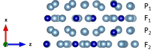
Figure 1: o-Al 13 Co 4 : Bulk structure showing a periodic stacking of two types of atomic planes: flat ( F ) and puckered ( P ). Co and Al atoms are represented by dark and light blue balls, respectively. Four planes perpendicular to the pseudo-10-fold [100] direction ( x direction) appear in a sequence P 1 F 1 P 2 F 2 (see text).
