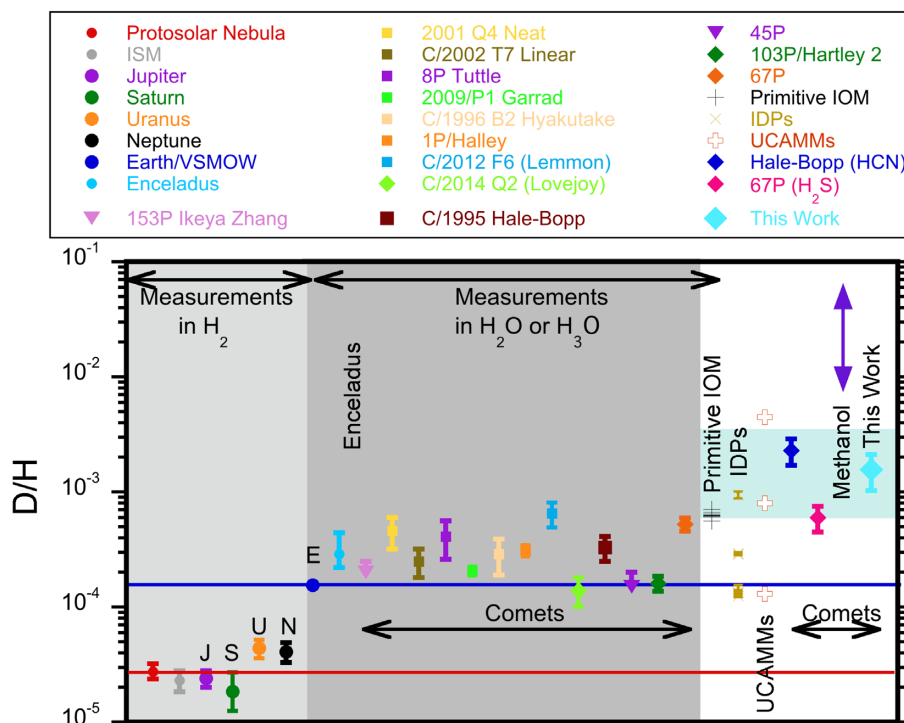
Figure 7. The D/H isotopic ratio measured in this work compared to that in the protosolar molecular cloud and the local interstellar medium (Ceccarelli et al. 2014) and in various objects in the Solar system, including the Earth (De Laeter et al. 2003), primitive IOM from meteorites (Alexander et al. 2012), bulk values for interplanetary dust particles (IDPs; Aléon et al. 2001; Messenger et al. 2003), ultracarbonaceous Antarctic micrometeorites (UCAMMs; Duprat et al. 2010), Jupiter and Saturn (Ceccarelli et al. 2014), Saturn’s moon Enceladus (Ceccarelli et al. 2014), Uranus and Neptune (Ceccarelli et al. 2014), Oort-Cloud comets (Ceccarelli et al. 2014; Altwegg et al. 2017), and Jupiter-family comets (Ceccarelli et al. 2014; Altwegg et al. 2017; Drozdovskaya et al. 2021). Measurements in H_2 are grouped to left (light-grey-shaded area), measurements in water or hydronium are in the middle (dark-grey-shaded area), and measurements in organics and H_2S are grouped to the right. The light blue box shows the range of ratios measured in the dust particles. The D/H ratio of the gas giants agree with the protosolar value, and ice giants are but little higher. Inner Solar system objects like the Earth have a higher value, but comets show a range of values (as do IDPs which may be of cometary origin). The OCCs were once thought to have higher D/H than the JFCs, but more recent measurements have invalidated this picture. The high D/H value in the HCN from comet Hale-Bopp is similar to the results of this work, which were also measured in organics. The D/H in methanol from comet 67P is even higher, greater than the highest results seen in refractory organics. The D/H ratio measured in the most primitive IOM is significantly lower than that seen in cometary organics and comparable to the higher values measured in UCAMMs.
