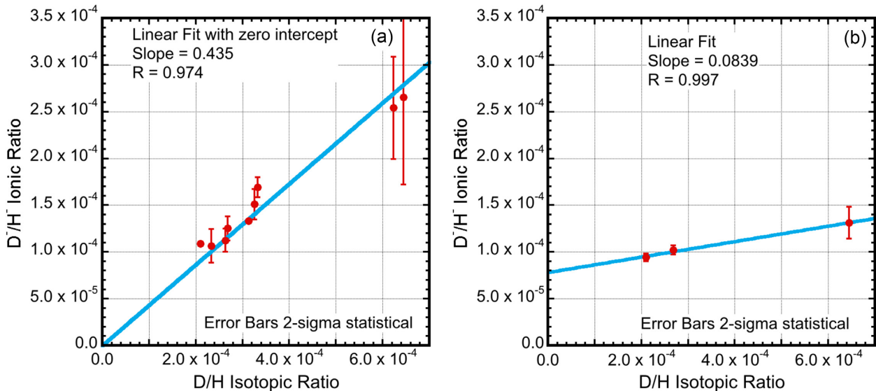
Figure 5. The results of measuring some of the IOM samples provided by Carnegie in another SIMS apparatus, a commercial IonToF 4 with a Bi^{3+} beam. Both panels show the D^-/H^- ionic ratios plotted versus the D/H isotopic ratio measured for the samples at Carnegie. Panel (a) shows the ionic ratio prior to sputtering (compare to Fig. 1b, above). The slope is 0.435, implying an IMF of 2.30, not dissimilar to the value derived for COSIMA of 3.19. Panel (b) shows the ionic ratio after sputtering. The slope of 0.0839 is much decreased, implying a greatly increased IMF of 11.9.
