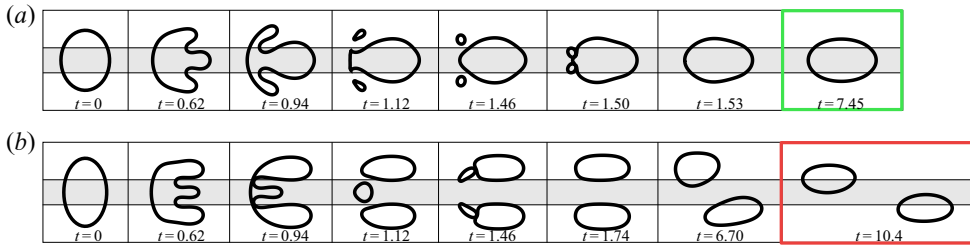
Figure 14. Numerical time evolutions of an initially centred elliptical bubble with parameters Q = 0.07 and d = 0.60 ( \Delta ) (a) and Q = 0.10 and d = 0.68 ( \nabla ) (b); see figure 13. The dimensionless time is given at the bottom of each snapshot. The bubble size is r = 0.54 .
