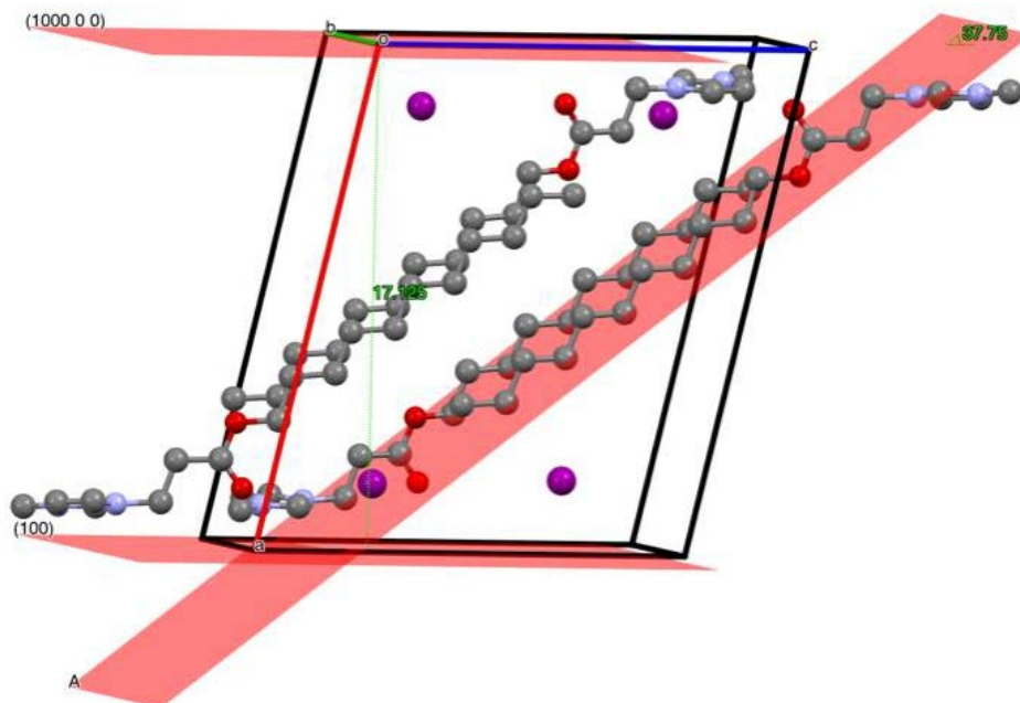
Figure S82: The crystal structure of [C_{11:0}E_{(2)}ImMe]I at 25 °C. The distance between the plan (1 0 0) and (1000 0 0) provide the layer distance, d_{Cr} = 17.1 Å. The plan A, formed by symmetrical alkyl chains, intersect plan (1 0 0) and (1000 0 0) with an angle, \alpha = 37.75^\circ . Thus, the tilt angle of the alkyl chains as compared to the layer normal is, \theta = 90^\circ - \alpha \sim 52^\circ
