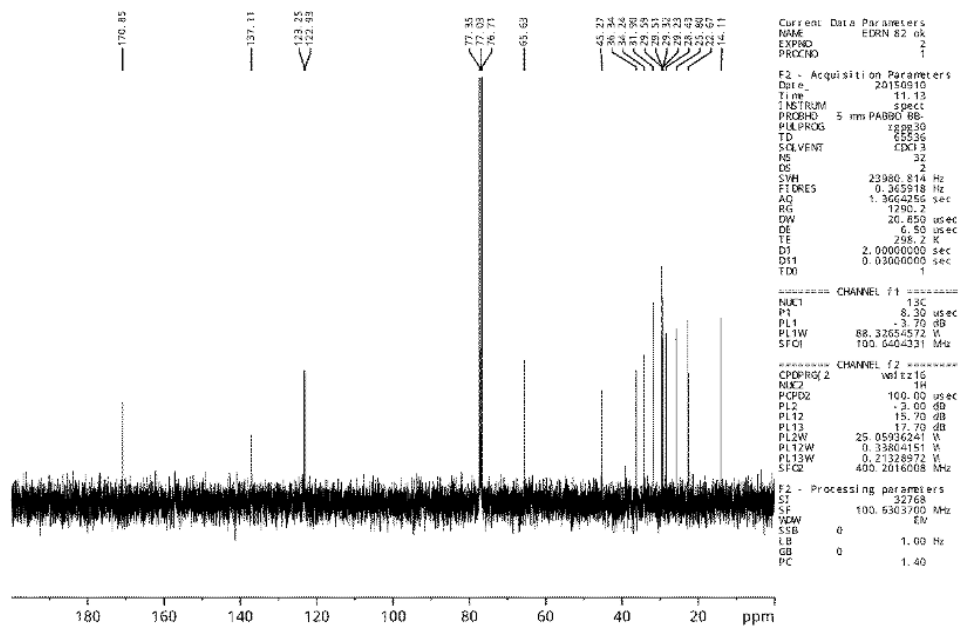
Figure S19: ^1\text{H} NMR spectrum (up) and ^{13}\text{C} NMR spectrum (down) in \text{CDCl}_3 of [\text{C}_{11:0}\text{E}_2]\text{Im}^+\text{BF}_4^-
