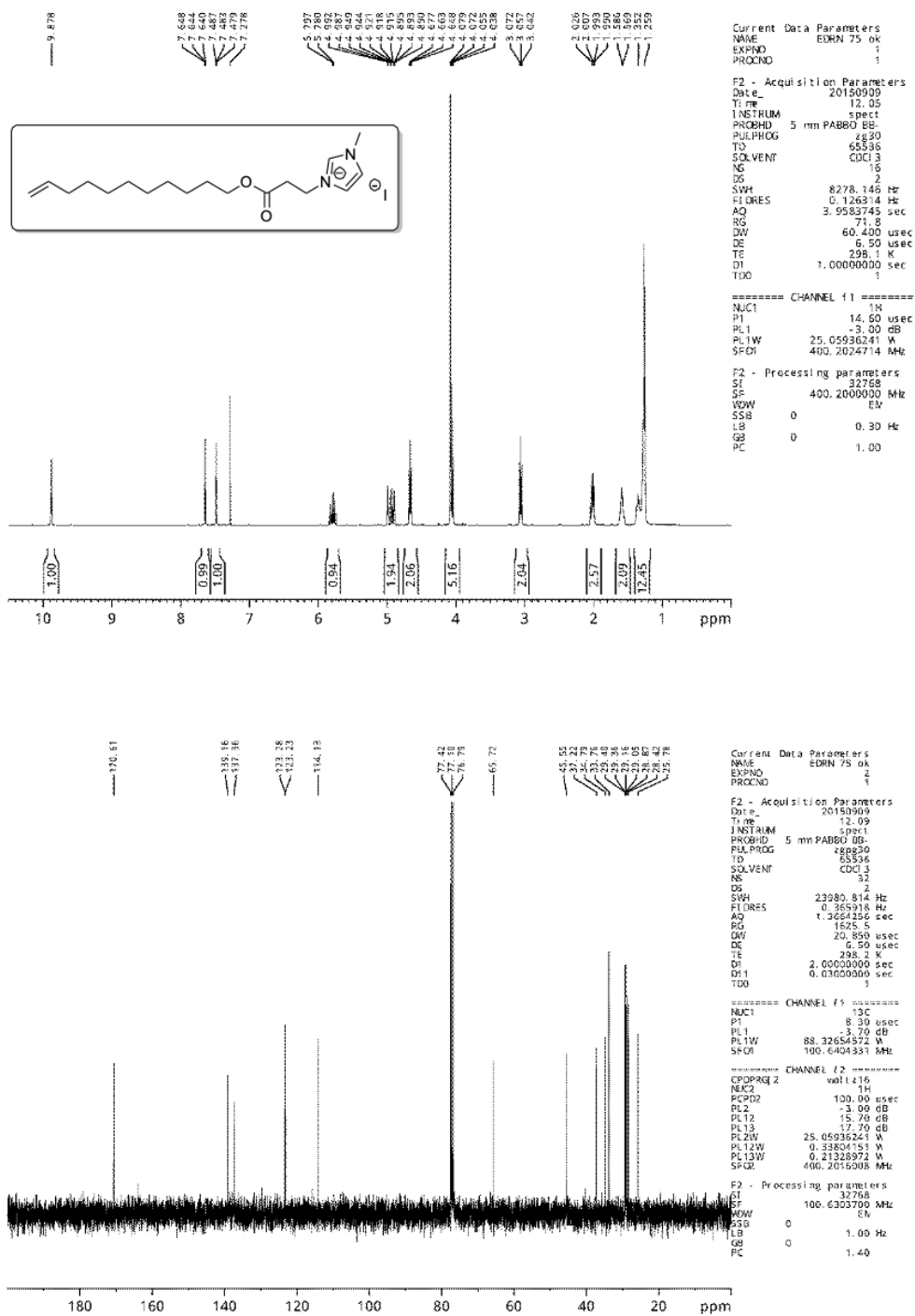
Figure S15: 1 H NMR spectrum (up) and 13 C NMR spectrum (down) in CDCl 3 of [C 11:1 E 2 ]Im]
