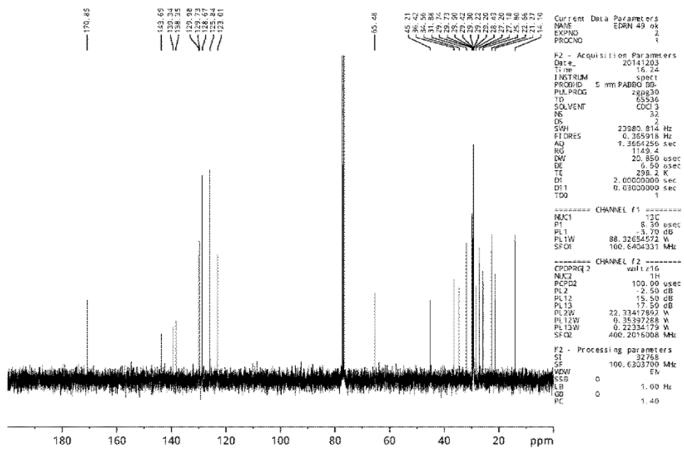
Figure S12: ^1H NMR spectrum (up) and ^{13}C NMR spectrum (down) in CDCl_3 of [C_{18:1E(2)}Im]pTsO
