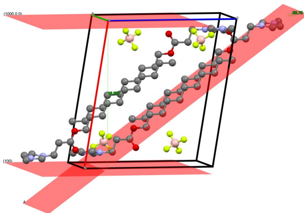
Figure S86: The crystal structure of [C_{11:0}E_{(2)}\text{ImMe}]\text{BF}_4 at 25 °C. The distance between the plan (1 0 0) and (1000 0 0) provide the layer distance, d_G = 17.0 Å. The plan A, formed by symmetrical alkyl chains, intersect plan (1 0 0) and (1000 0 0) with an angle, \alpha = 36.79^\circ . Thus, the tilt angle of the alkyl chains as compared to the layer normal is, \theta = 90^\circ - \alpha \sim 53^\circ
