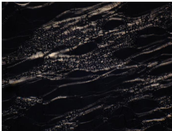
Figure S63: Optical microscopic texture of the mesophase (Smectic A) observed under crossed polarizers at elevated temperature for [C_{18:0}E_{(2)}ImMe]pTsO ( T_m = 81 °C, T_{LC} = 172 °C), T = 100 °C (oily streak texture).
