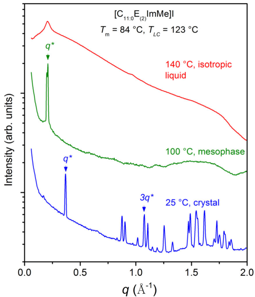
Figure S72: Small angle X-ray scattering patterns for [C_{11:0}E_{(2)}ImMe]I ( T_m = 84 °C, T_{LC} = 123 °C) in the crystal (25 °C), the SmA (100 °C) and isotropic (140 °C) phases. The patterns were acquired during a heating cycle. In the crystal phase and the mesophase the principal scattering peak ( q^* ) and the higher order reflection peaks (multiple of q^* ) are indicated by pointed down triangles.
