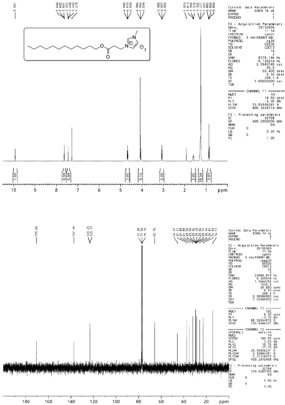
Figure S16: ^1\text{H} NMR spectrum (up) and ^{13}\text{C} NMR spectrum (down) in \text{CDCl}_3 of [\text{C}_{12:0}\text{E}(2)\text{Im}]\text{I}
