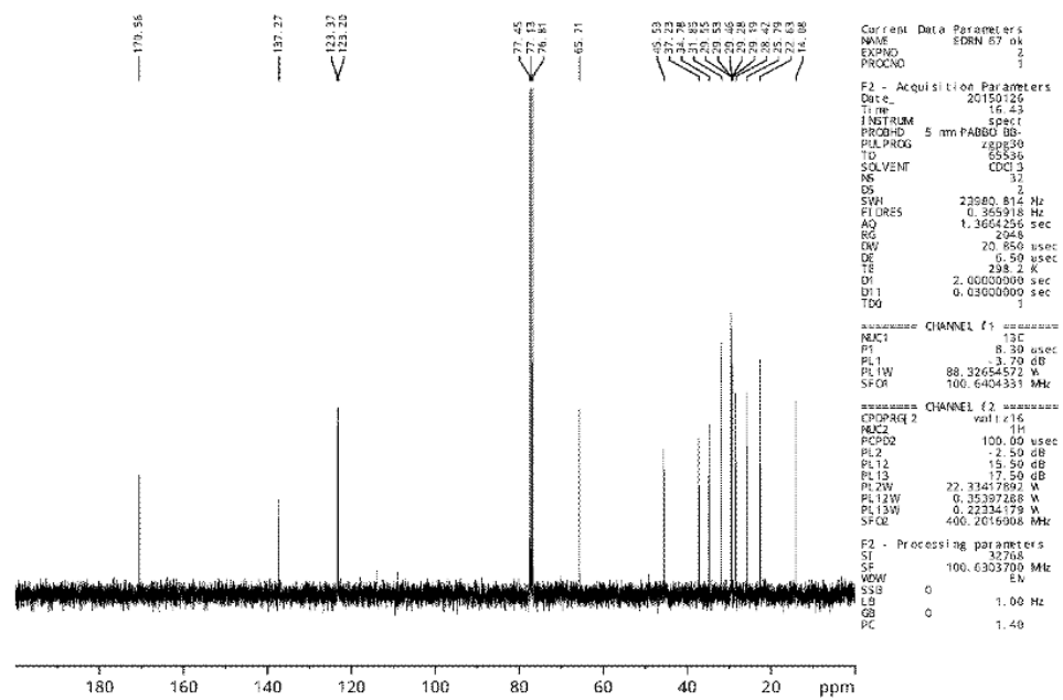
Figure S14: 1 H NMR spectrum (up) and 13 C NMR spectrum (down) in CDCl 3 of [C 11:0 E (2) Im]
