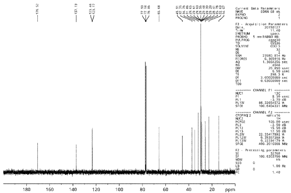
Figure S17: ^1\text{H} NMR spectrum (up) and ^{13}\text{C} NMR spectrum (down) in \text{CDCl}_3 of [C_{18:0}E_{(2)}Im]
