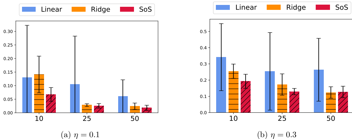
Figure 3: Mean square error (MSE) of functions fitted using convex piecewise linear regression, kernel ridge regression and kernel convex sum-of-squares regression on 2D data generated according to eq. (30) with a = 1 , as a function of noise ( \eta ) and number of samples (x-axis). Full bars represent averaged scores over 10 runs, error bars correspond to plus/minus standard deviation.
