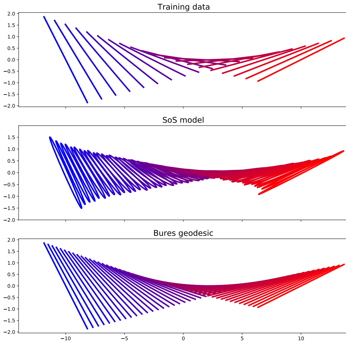
Figure 6: Interpolation of a rank 1 Bures geodesic from 12 data points (top). The matrices are represented as the level sets of (potentially degenerate) Gaussian distributions: \{x : \mathcal{N}(x; 0, \Sigma) \leq r\} . We use the exponential kernel and select all hyperparameters using cross-validation. The learned model is represented in the middle figure, and the full geodesic is plotted in the bottom figure for comparison.
