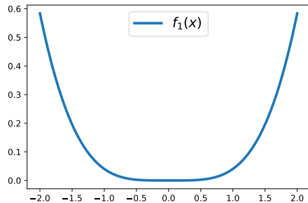
Figure 2: Ground truth (1D)
