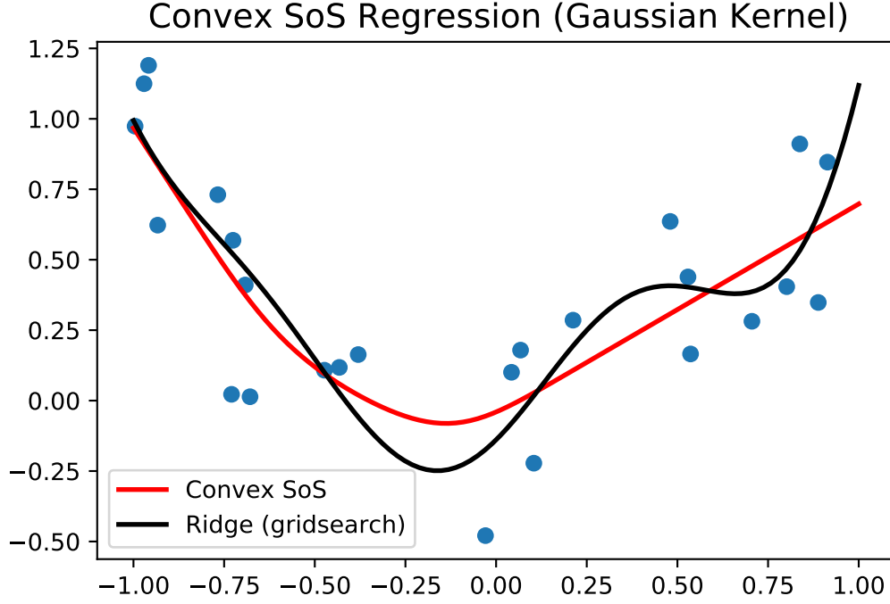
Figure 5: Convex regression with reproducing property: 1D example.
