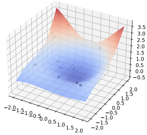
(b) Kernel ridge regression
