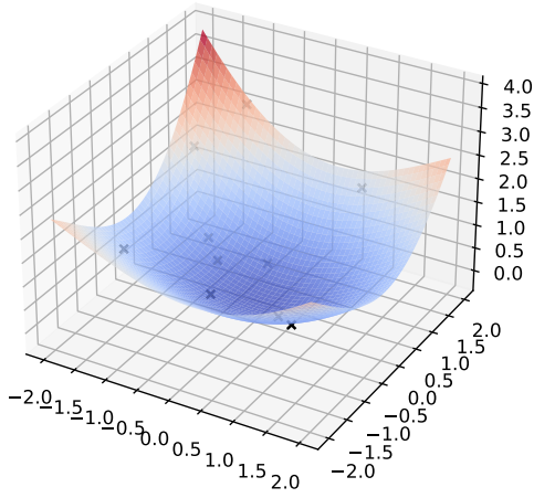
(a) Kernel SoS
