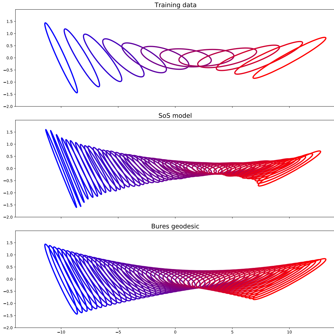
Figure 1: Interpolation of a Bures geodesic from 12 data points (top). The matrices are represented as the level sets of Gaussian distributions: \{x : \mathcal{N}(x; 0, \Sigma) \leq r\} for r = 0.1 . We use the exponential kernel and select all hyperparameters using cross-validation. The learned model is represented in the middle figure, and the full geodesic is plotted in the bottom figure for comparison.
