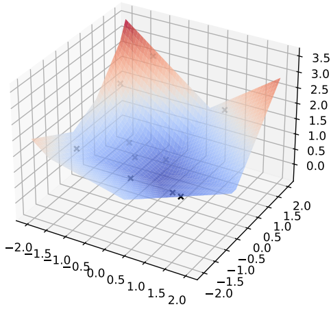
(c) Piecewise linear convex regression
