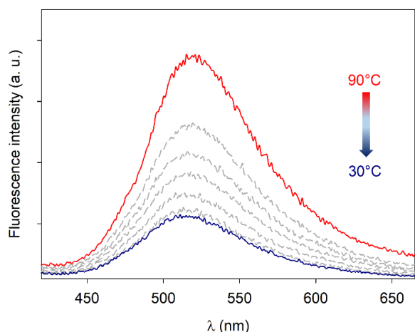
Figure 14. Evolution of the emission spectrum of a \text{C}_3\text{Pyr} -TCNQ- \text{F}_4 (3 equiv.) mixture as a function of temperature ( [\text{C}_3\text{Pyr}] = 8 \text{ mg}\cdot\text{mL}^{-1} , TCE, \lambda_{\text{exc}} = 344 \text{ nm} ; interval of 10 K between each curve).
