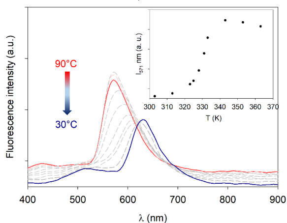
Figure 15. Evolution of the emission spectrum of a \text{C}_3\text{Pyr} -NDI (3 equiv.) mixture as a function of temperature ( [\text{C}_3\text{Pyr}] = 8 \text{ mg}\cdot\text{mL}^{-1} , TCE, \lambda_{\text{exc}} = 344 \text{ nm} ). Inset: Corresponding evolution of the emission intensity at 571 nm as a function of temperature.
