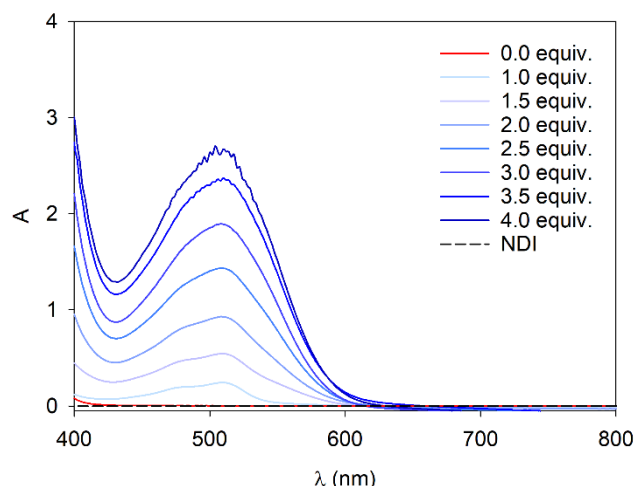
Figure 10. Evolution of the UV-visible absorption spectrum of \text{C}_3\text{Pyr} ( 8\text{ mg}\cdot\text{mL}^{-1} , 5.2\text{ mM} in TCE, 293\text{ K} ) upon addition of NDI acceptor. The scattering was corrected by subtracting the absorbance at 800\text{ nm} .
