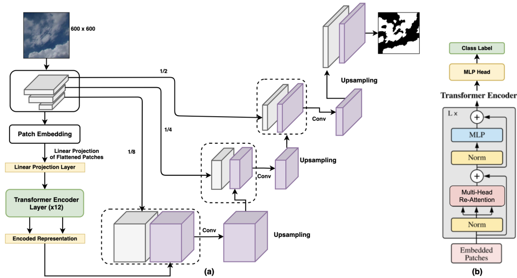
Figure 1: (a) Cloud U-Net Transformer (CloudUT) (b) Cloud Vision Transformer (CloudViT)
