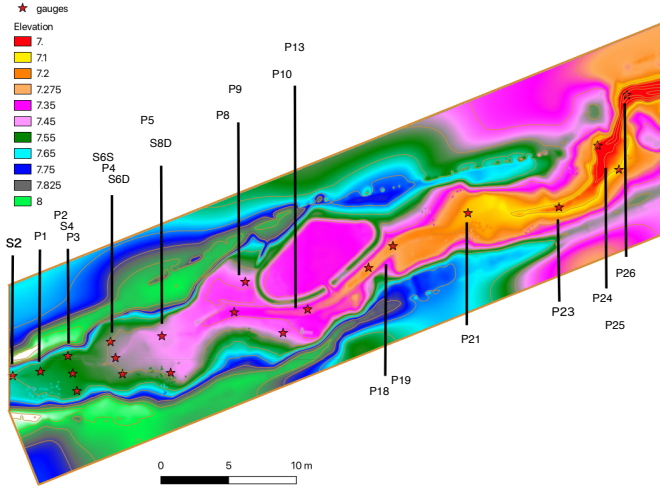
Figure 7. Topography of the fluvial case with position and name of the gauge stations. The inflow is coming from the left border of the domain. Figure 8. Hydrograph of the imposed inflow on the left boundary.
