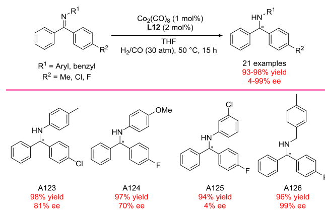
Scheme 72. The first Co-catalyzed hydrogenation of imines.
