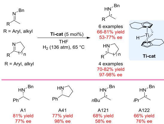
Scheme 70. Buchwald's system for imines asymmetric hydrogenation.
