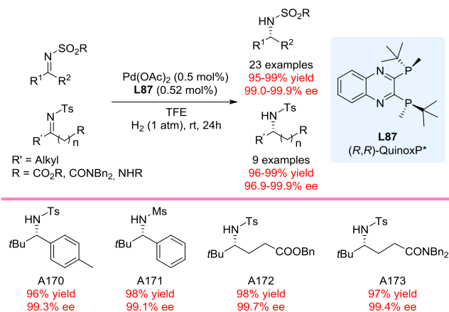
Scheme 92. Asymmetric hydrogenation of sulfonyl imines with QuinoxP* ligand.
