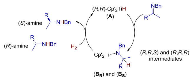
Scheme 71. Proposed mechanism for Ti(III) hydride catalyzed imines hydrogenation.
