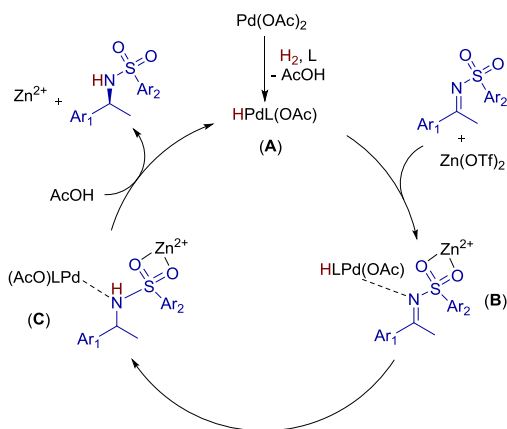
Scheme 90. Proposed mechanism for the Pd-Zn co-catalyzed hydrogenation.
