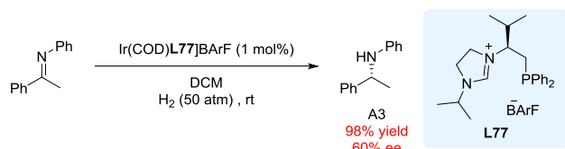
Scheme 69. Ir-NHC system for the hydrogenation of an imine.
