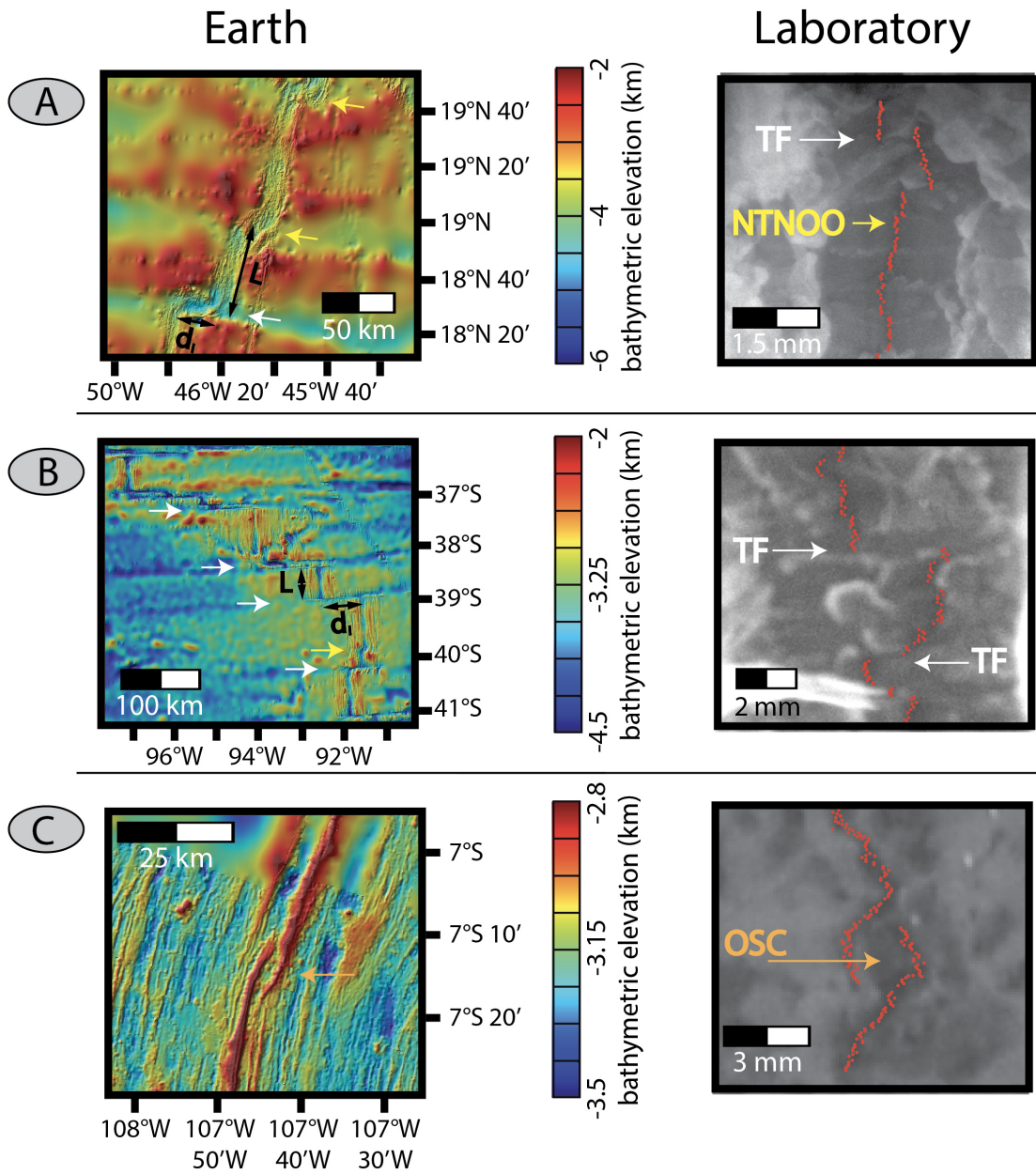
Figure 1: Zoology of discontinuities observed on Earth (left panels) and reproduced in the laboratory (right panels) including examples of non-transform non-overlapping offset, NTNOO, see text (A), transform fault, TF (B) and overlapping spreading centre, OSC (C). The small red dots indicate the axis location determined by the image local intensity minima.
