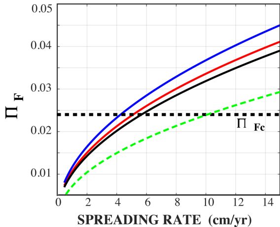
Figure 4: Evolution of \Pi_F (equation (3)) as a function of spreading velocity for different mantle temperatures and thermal diffusivities. The solid lines are for \kappa_T=10^{-6} \text{m}^2/\text{s} ; the dashed lines are for \kappa_T=2.10^{-6} \text{m}^2/\text{s} . In blue, T_m=1600^\circ\text{C} ; in red and in green, T_m=1400^\circ\text{C} ; in black, T_m=1300^\circ\text{C} .
