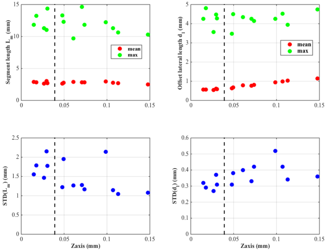
Figure A.10: Experimental data as a function of the axial elastic thickness. The black dashed line corresponds to \Pi_F = \Pi_{F_C} . STD stands for standard deviation. For each experiment, the average value of segment length and of offset size are in red, while their maximum values are in green.
