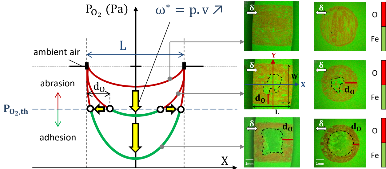
Fig.1. Illustration of the contact oxygenation concept (COC) showing the transition from pure abrasive to a mixed abrasive-adhesive wear and application of the latter on flat circular [13] and square [12] shaped fretting interfaces as reflected by the EDX maps.
