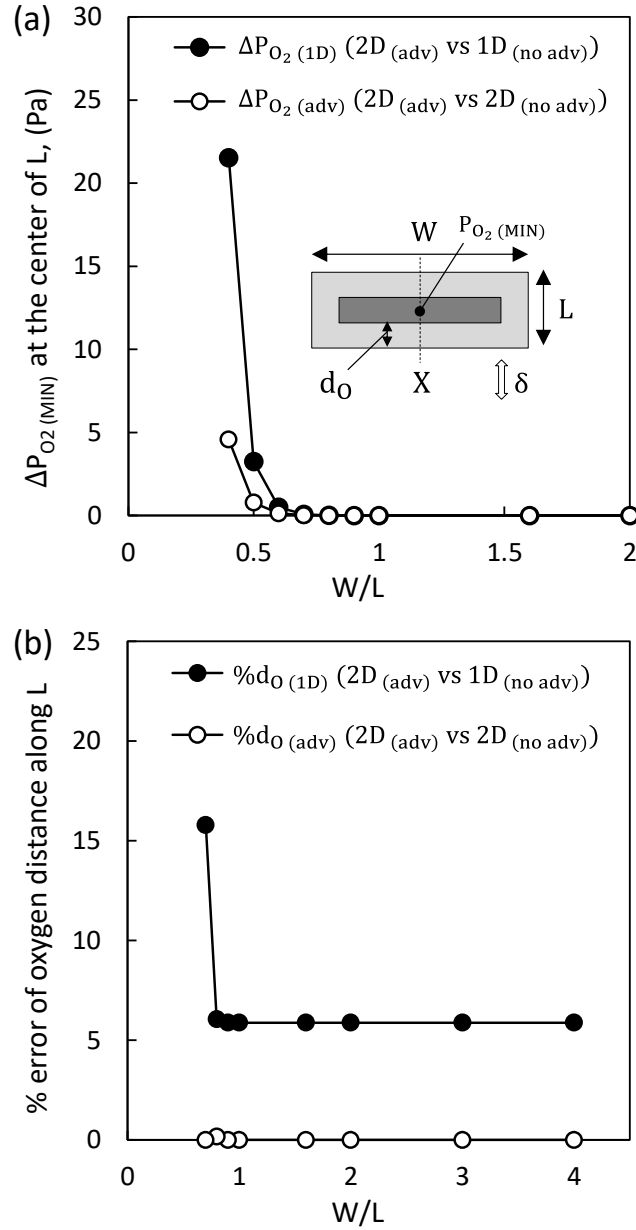
Fig.3. (a) Evolution of \Delta P_{O_2(1D)} and \Delta P_{O_2(adv)} index errors versus W/L ratio; (b) evolution of \% d_{O(1D)} and \% d_{O(adv)} index errors versus W/L ratio estimated for a nonzero adhesion zone ( p=100 MPa, \delta_g=\pm 100 \mu\text{m} , and f=1 Hz).
