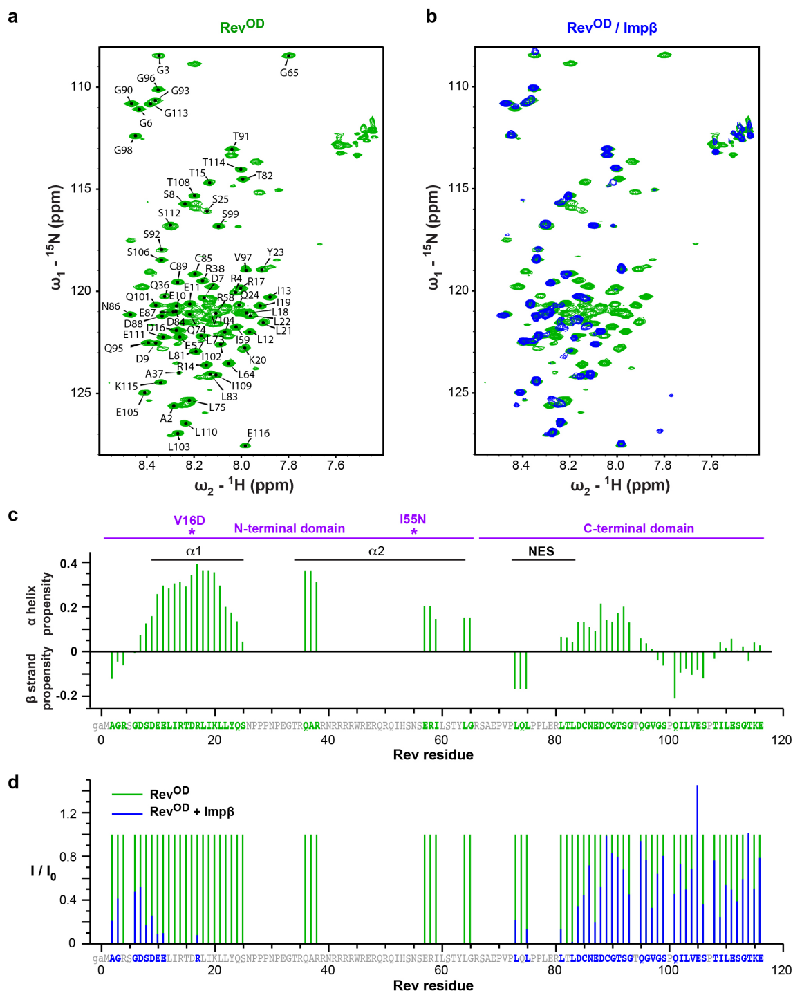
Figure 4. NMR analysis of Rev binding by Impβ. a. ^1\text{H}, ^{15}\text{N} HSQC spectrum of free Rev OD (600MHz, 283K). b. ^1\text{H}, ^{15}\text{N} -HSQC spectrum Impβ-bound Rev OD (blue) superimposed on that of unbound Rev OD (green). c. Secondary chemical shifts 127 of unbound Rev OD . The two point mutations are indicated by asterisks. d. Ratio of peak intensities for Rev residues in the presence and absence of Impβ (600MHz, 283K).
