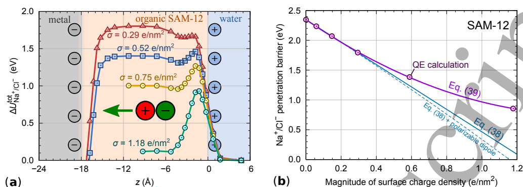
Figure C.2. (a) QE calculated energy profiles for the penetration of the \text{Na}^+/\text{Cl}^- ion-pair from water through SAM-12 toward the metal surface for several metal surface charge densities \sigma . Note the emergence of “extra solvation energy penalty” as the magnitude of metal surface charge density increases. (b) QE calculated activation energies (data points) for the penetration of \text{Na}^+/\text{Cl}^- ion-pair through SAM-12 as a function of metal surface charge density. The fit of QE data points with Eq. [41] is indicated by purple line, whereas bluish line indicates the prediction of Eq. [40]; the case of polarizable \text{Na}^+/\text{Cl}^- dipole, Eq. [C.3], is indicated by dashed curve, where the PBE calculated value of \alpha = 30 \text{ Bohr}^3 was taken for the polarizability of the \text{Na}^+/\text{Cl}^- ion-pair.
