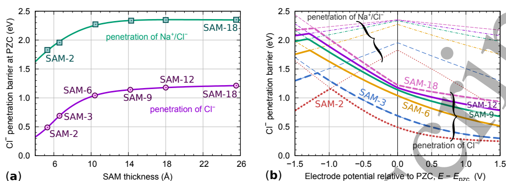
Figure 16. (a) Activation barriers for the penetration of standalone Cl - (purple) and of the Na + /Cl - ion-pair (cyan) at PZC as functions of the SAM thickness. (b) Activation barriers for the penetration into SAM- x with x \in \{2, 3, 6, 9, 12, 18\} as functions of the electrode potential (relative to PZC). The activation barriers for both the standalone Cl - ion and the Na + /Cl - ion-pair are considered, where the former are calculated by Eq. [33] and the latter by Eq. [41].
