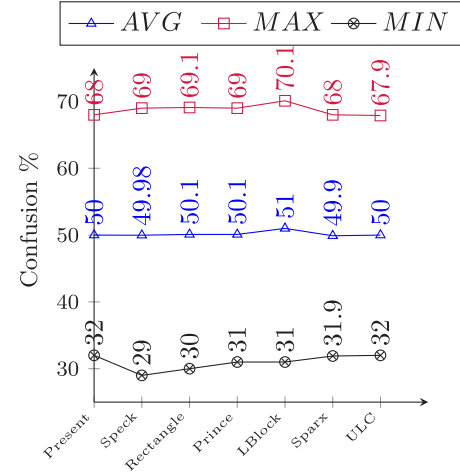
Fig. 8. Evaluation of confusion level of our cryptosystem (ULC) and the existents lightweight cryptosystems.
