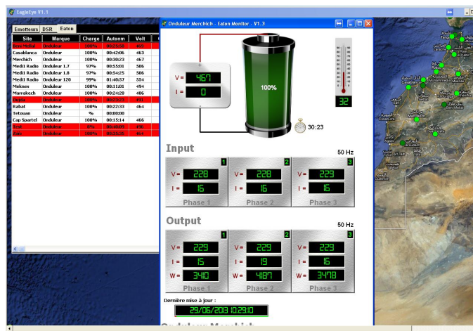
Fig 4: example of (inverted variables make Eaton) measurements of equipment device (Powerware 9355-20KVA UPS) after verification of WN by means of RTT
