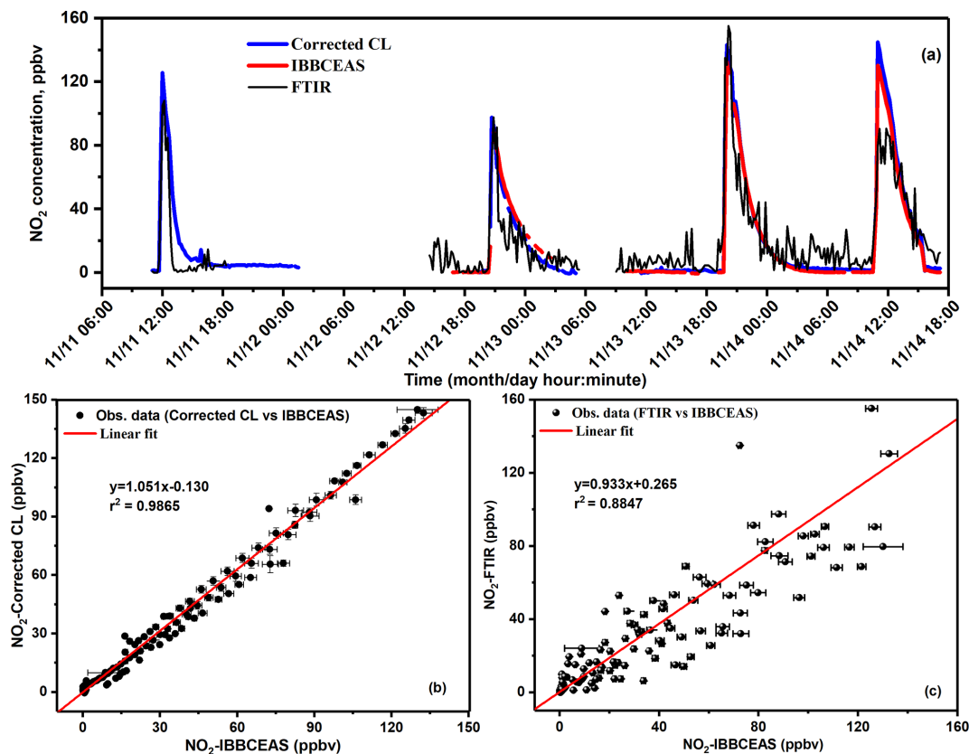
Figure 7. (a) Intercomparison measurement for NO 2 detection between IBBCEAS, FTIR and NO x analyser after HONO interference correction; (b) correlation of the measured NO 2 concentrations between UV-LED-IBBCEAS and NO x analyser (CL) with HONO interferences correction; (c) correlation of the measured NO 2 concentrations between UV-LED-IBBCEAS and FTIR.
