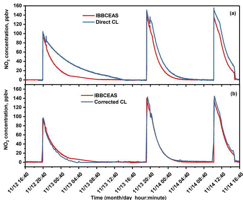
Figure 6. Investigation of positive interferences from nitrogen-containing species (here HONO) in the NO x analyser (CL) measurement in comparison to the UV-LED-IBBCEAS measurement: (a) from CL-NO x analyser without HONO correction; (b) CL-NO x analyser results after HONO correction.
