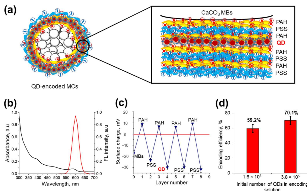
Figure 4. Obtaining microcapsules optically encoded with quantum dots (QDs). (a) A schematic diagram of the arrangement of the QD and PAH/PSS layers in the polyelectrolyte shell. (b) Optical characteristics of the CdSe/ZnS core/shell QDs solubilized with a PEG derivative (HS-(PEG) 12 -COOH). (c) Changes in the \zeta -potential of the microbead/microcapsule surface upon application of the PAH/PSS polyelectrolytes and QD layers. (d) Estimated efficiency of the optical encoding of the microcapsules.
