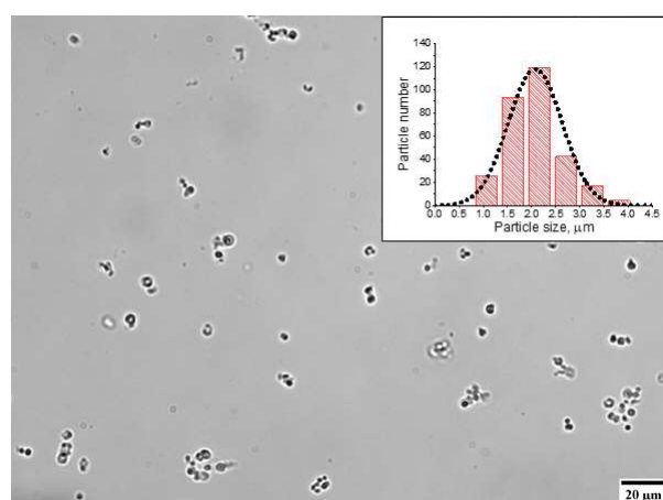
Figure 2. Microphotograph of typical polyelectrolyte microcapsules obtained by optical microscopy. The size distribution histogram of the prepared microcapsules is shown in the inset.
