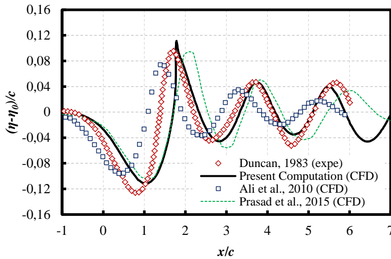
Figure 5 – Comparison of free-surface deformations between experimental data from Duncan 1983 (Duncan 1983), numerical data from Ali et al., 2010 (Ali and Karim 2010) and Prasad et al., 2015 (Prasad, Hino, and Suzuki 2015) and the present computation for h/c = 0.911 . The hydrofoil is located under the free-surface between x/c = 0 and x/c = 1 .
