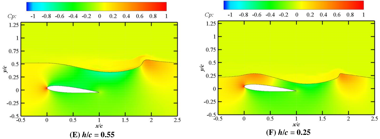
Figure 7 – Hydrodynamic pressure field around the NACA0012 for different submergence depth to chord ratios, an angle of attack of 5^\circ and a chord-based Froude number of 0.571. (The hydrostatic pressure has been subtracted.)
