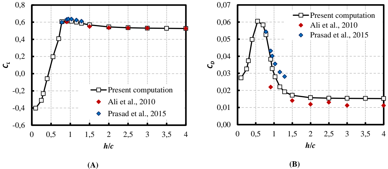
Figure 6 – Comparison of (A) lift coefficients and (B) drag coefficients between numerical data from Ali et al., 2010 (Ali and Karim 2010) and Prasad et al., 2015 (Prasad, Hino, and Suzuki 2015) and the present computation. (Note that the results at h/c = 0.1 are not considered reliable.)
