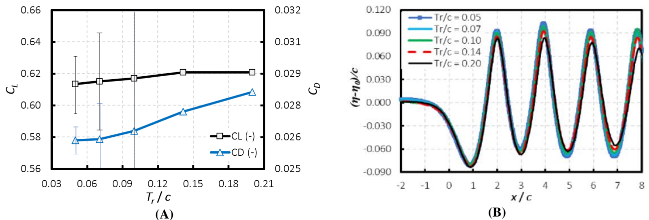
Figure 3 - Grid convergence with respect to the grid refinement threshold T_r/c (the lower the threshold, the finer the mesh) of (A) lift and drag coefficients and (B) free-surface deformation.
