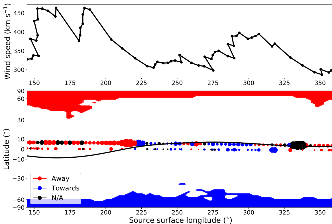
Fig. 3. Overview of the HCS location and orientation. Bottom panel: Map of the Sun’s source surface, at 2.5 R_{\odot} , with the red/blue contours showing open field lines with positive/negative polarity using an Air Force Data Assimilative Photospheric Flux Transport (ADAPT; Worden & Harvey 2000) magnetogram on June 1, 2020. The neutral line is shown as a solid black line, which is used as a proxy for the HCS. Overlain is a 6-hour average of the in situ magnetic field data from Wind (lower) and Solar Orbiter (upper), mapped back to the source surface using a ballistic procedure. The color of these points represents the polarity, which has been defined as being within \pm 45^{\circ} of the Parker spiral direction at each spacecraft. If the field direction lay outside this range then it has been not assigned a polarity (N/A). To signify changes in magnitude of the magnetic field B , the areal size of the points is proportional to B^2 , normalized by the radial distance to the Sun. The two ICMEs can be seen at 220^{\circ} , where the point size increases along with a change in magnetic polarity. On this plot the spacecraft travels from right to left. Top panel: Solar wind speed measured by the Wind spacecraft, mapped back to the solar source surface. This reveals a positive polarity HSS between 150^{\circ} and 200^{\circ} longitude, preceded by a negative polarity slower plasma flow.
